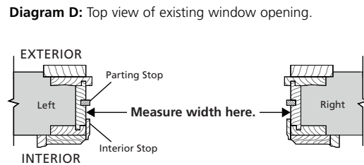
Diagram D: Top view of existing window opening.
