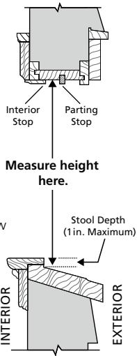
Diagram B: Side view of existing window opening.
