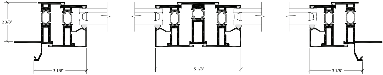
OUTSIDE GLAZED DOUBLE CASEMENT
