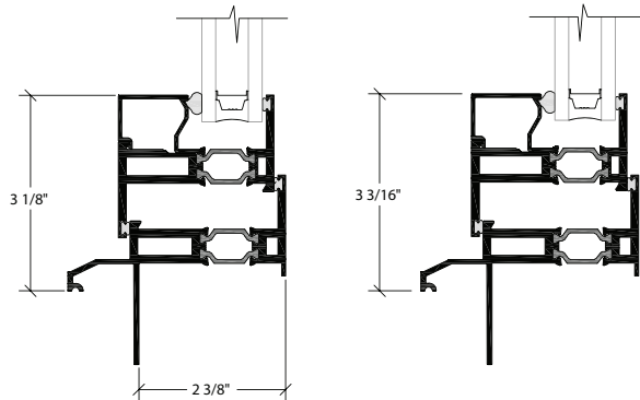
OUTSIDE GLAZED FIXED OVER AWNING
