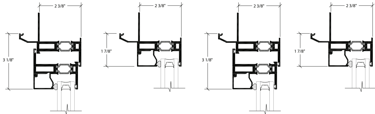
OUTSIDE GLAZED DOUBLE CASEMENT
