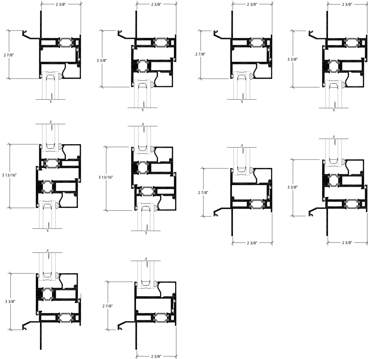
INSIDE GLAZED FIXED OVER AWNING
