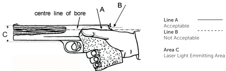
Figure 5. Laser Hit&Miss Target (examples)
