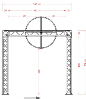
BIG WHEELS - SIDE VIEW Scale: 1:20
