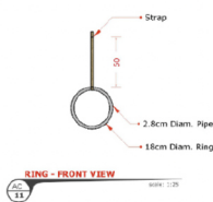
RINGS - FRONT VIEW SCALE: 1:100
