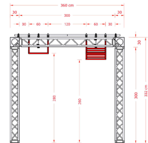
LADDERS - FRONT VIEW scale: 1:25
