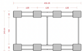
STEPS - PLAN VIEW Scale: 1:30
