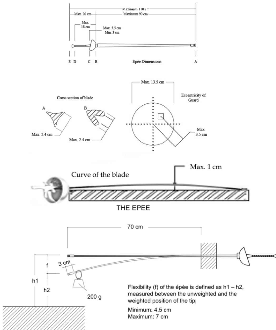
Figure 9. Épée dimensions and flexibility
