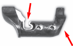
Magazine Catch Removed From Pistol - To Show Notch for Spring Rod
