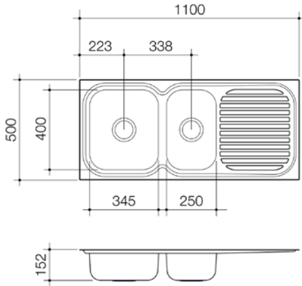
RADIANT 1100MM 1.75EB 1TH LHB R150.1L
