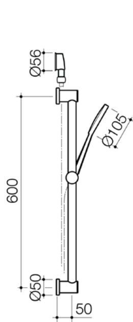
ROUND BASIC RAIL SHOWER CL10058.C3A CHROME
