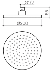
CLARK RND II OVER HEAD SHOWER 200MM WELS 3 star rated, 9L/min CL10076.C3A CHROME CL10076.B3A BLACK CL10076.BN3A BRUSHED NICKEL
