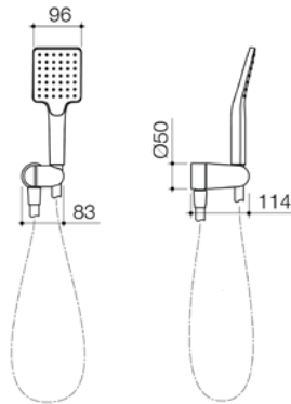
BASIS SQUARE HAND SHOWER WELS 3 star rated, 9L/min BAS034C3A CHROME BAS034B3A BLACK BAS034BN3A BRUSHED NICKEL
