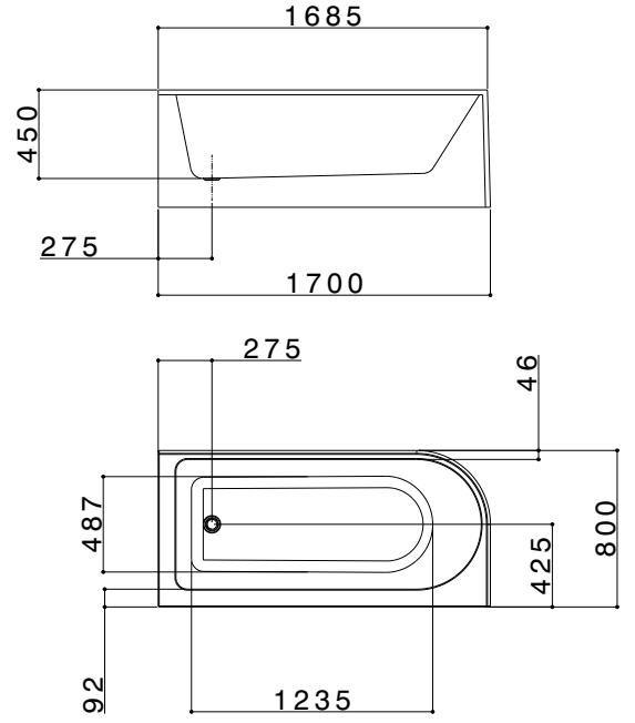
ORIGIN 1700 RIGHT HAND CORNER BATH OR7RHCW
