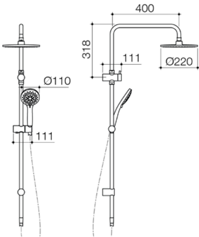
BASIS ROUND RAIL SHOWER W/OVERHEAD WELS 3 star rated, 9L/min BAS033C3A CHROME BAS033B3A BLACK BAS033BN3A BRUSHED NICKEL
