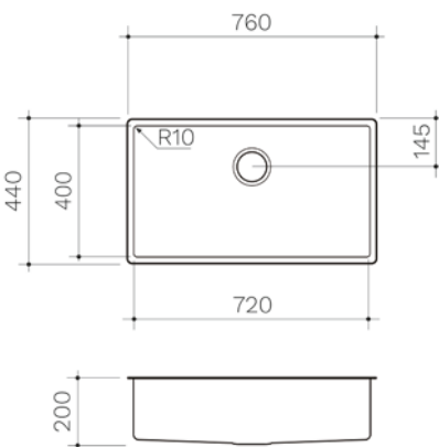
PRISM LARGE SINGLE BOWL OVERMOUNT/UNDERMOUNT PPR10LGB
