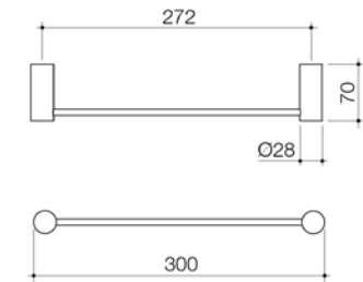
BASIS HAND TOWEL RAIL BAS043C CHROME BAS043B BLACK BAS043BN BRUSHED NICKEL
