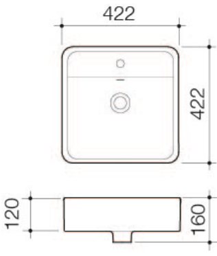
STYLUS BASIS SQUARE INLET BASIN BAS0815W
