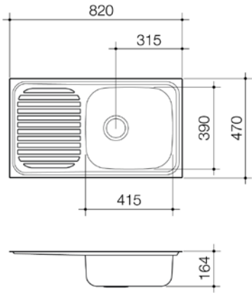
RADIANT R110 SINGLE END BOWL 1TH RHB R110.1R
