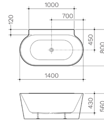
CLARK RND 1400 BTW F/S BATH OF CL50003.WBTW
