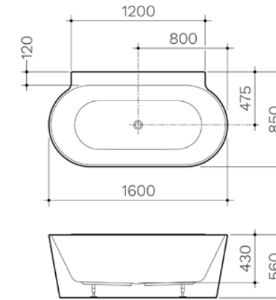
CLARK RND 1600 BTW F/S BATH OF CL50004.WBTW
