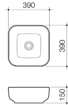
TRIBUTE ABOVE COUNTER BASIN - SQUARE 390MM 874400W
