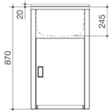
UTILITY 42L COMP T/C BP F6111
