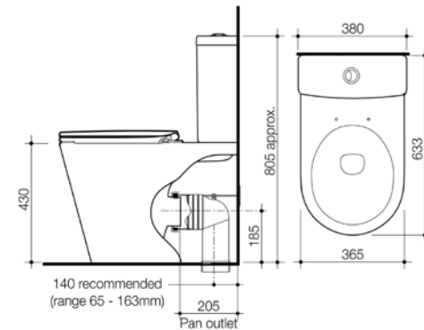
STYLUS ORIGIN RIMLESS BACK-TO-WALL TOILET SUITE BI/BE (WITH ADAPTER) WELS 4 Star Rated, 4.5/3L OR001
