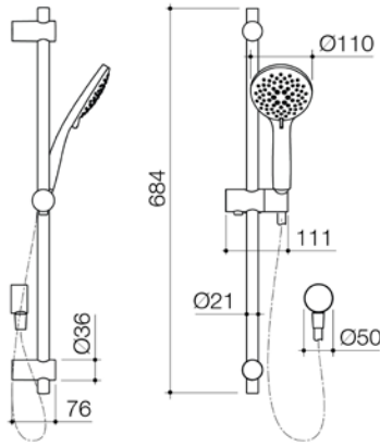
BASIS ROUND RAIL SHOWER WELS 3 star rated, 9L/min BAS032C3A CHROME BAS032B3A BLACK BAS032BN3A BRUSHED NICKEL
