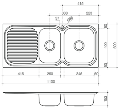
RADIANT 1100MM 1.75EB 1TH RHB R150.1R
