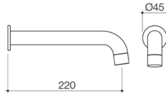
BASIS WALL BASIN/BATH OUTLET 220MM WELS 5 star rated, 6L/min BAS046C5AF CHROME BAS046B5AF BLACK BAS046BN5AF BRUSHED NICKEL
