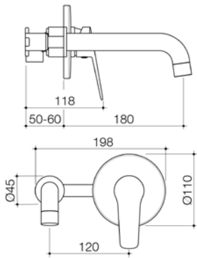
BASIS R4 WALL BASIN/BATH MIXER 180MM SPOUT BAS047C5AF CHROME BAS047B5AF BLACK BAS047BN5AF BRUSHED NICKEL
