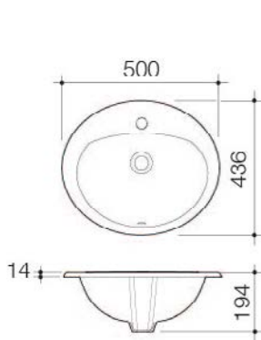
STYLUS BASIS VANITY BASIN BAS0615W
