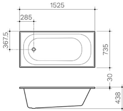
BASIS BATH 1525 4TF WHITE BB5W
