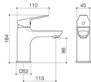
BASIS R4 BASIN MIXER BAS021C5AF CHROME BAS021B5AF BLACK BAS021BN5AF BRUSHED NICKEL
