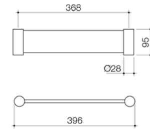
BASIS METAL SHELF 300MM BAS044C CHROME BAS044B BLACK BAS044BN BRUSHED NICKEL
