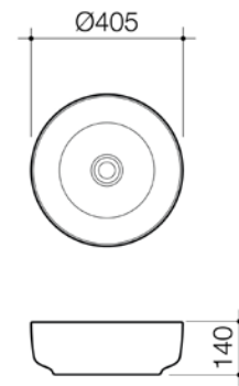
TRIBUTE ABOVE COUNTER BASIN - ROUND 405MM 874300W
