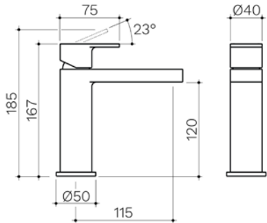
CLARK RND SQR BASIN MIXER LF CL10018.C5AF CHROME CL10018.B5AF BLACK
