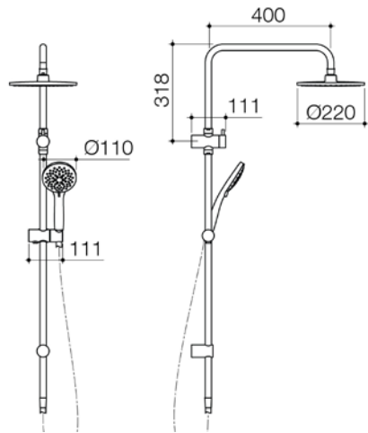
BASIS ROUND RAIL SHOWER W/OVERHEAD WELS 3 star rated, 9L/min BAS033C3A CHROME BAS033B3A BLACK BAS033BN3A BRUSHED NICKEL
