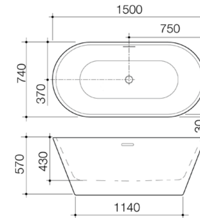
BASIS FREESTANDING 1500 BATH WITH OVERFLOW BB5FWOF
