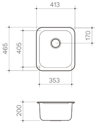
PRISM SINGLE BOWL UNDERMOUNT/OVERMOUNT PPR10B
