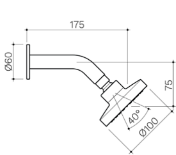
ROUND BASIC FIXED SHOWER WELS 3 star rated, 9L/min CL10056.C3A
