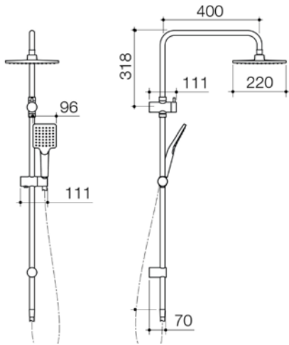
BASIS SQUARE RAIL SHOWER W/OVERHEAD WELS 3 star rated, 9L/min BAS036C3A CHROME BAS036B3A BLACK BAS036BN3A BRUSHED NICKEL
