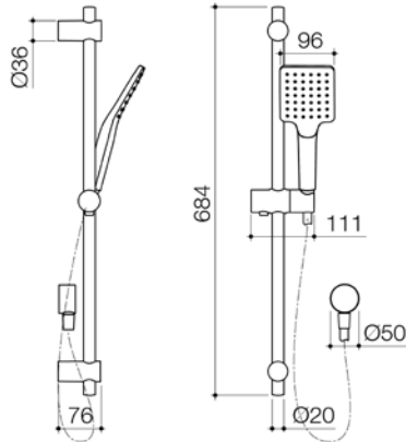
BASIS SQUARE RAIL SHOWER WELS 3 star rated, 9L/min BAS035C3A CHROME BAS035B3A BLACK BAS035BN3A BRUSHED NICKEL
