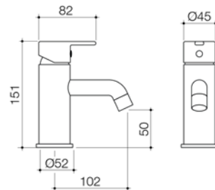
BASIS R2 BASIN MIXER WELS 5 star rated, 6L/min BAS017C5AF CHROME BAS017B5AF BLACK BAS017BN5AF BRUSHED NICKEL
