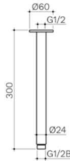
CEILING ARM 300MM CL10054.C CHROME CL10054.B BLACK CL10054.BN BRUSHED NICKEL
