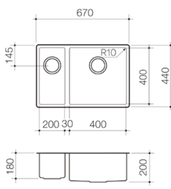
PRISM 1.5 RIGHT HAND BOWL UNDERMOUNT/OVERMOUNT PPR15BRH
