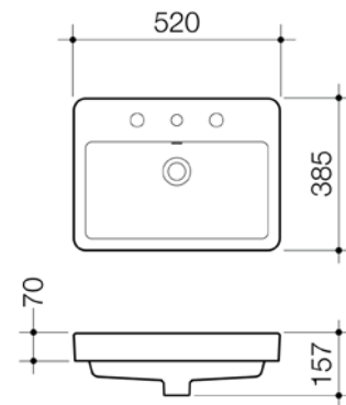
BASA INSET BASIN 1TH OF 633315W
