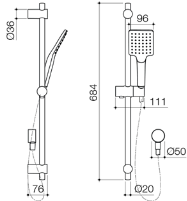
BASIS SQUARE RAIL SHOWER WELS 3 star rated, 9L/min BAS035C3A CHROME BAS035B3A BLACK BAS035BN3A BRUSHED NICKEL
