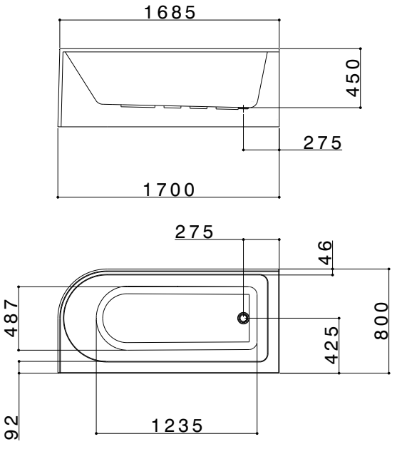
ORIGIN 1700 LEFT HAND CORNER BATH OR7LHCW
