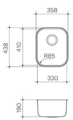
MONACO SINGLE BOWL OVERMOUNT EVB
