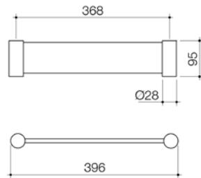
BASIS METAL SHELF 300MM BAS044C CHROME BAS044B BLACK BAS044BN BRUSHED NICKEL
