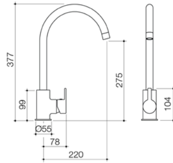
BASIS R2 SINK MIXER WELS 4 star rated, 7.5L/min BAS018C4AF CHROME BAS018B4AF BLACK BAS018BN4AF BRUSHED NICKEL
