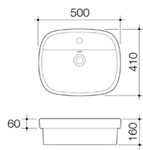
STYLUS BASIS RECTANGULAR INLET BASIN BAS0915W
