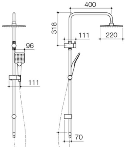
BASIS SQUARE RAIL SHOWER W/OVERHEAD WELS 3 star rated, 9L/min BAS036C3A CHROME BAS036B3A BLACK BAS036BN3A BRUSHED NICKEL
