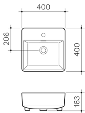
CLARK SQUARE 400 SEMI RECESSED BASIN 1TH OF
