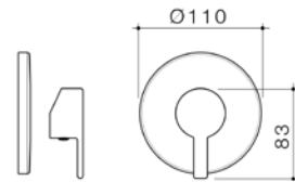
BASIS R2 B/S MIXER TRIM KIT BAS027C CHROME BAS027B BLACK BAS027BN BRUSHED NICKEL
