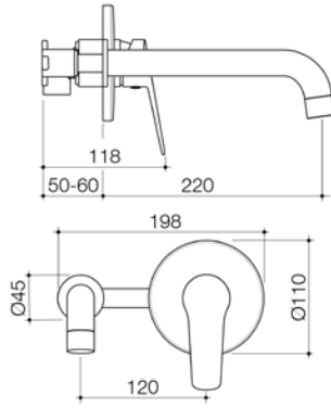
BASIS R4 WALL BASIN/BATH MIXER 220MM SPOUT BAS048C5AF CHROME BAS048B5AF BLACK BAS048BN5AF BRUSHED NICKEL
