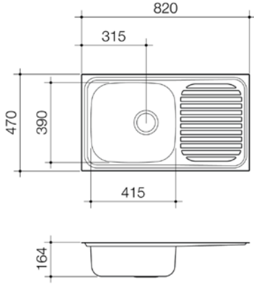
RADIANT R110 SINGLE END BOWL 1TH LHB R110.1L
