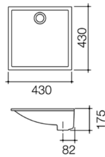
LIANO 430 UC VB NTH OF 664205W
