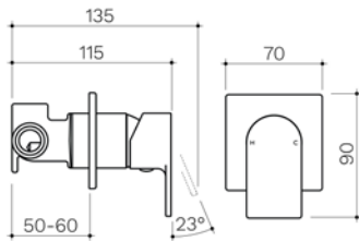
CLARK RND SQR W MXR SQR B/P CL10032.C CHROME CL10032.B BLACK
