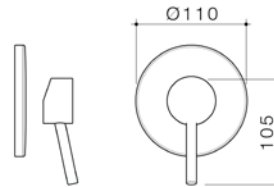
BASIS R3 B/S MIXER TRIM KIT BAS028C CHROME BAS028B BLACK BAS028BN BRUSHED NICKEL
