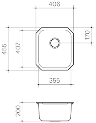
MONACO SINGLE BOWL UNDERMOUNT EVBU
