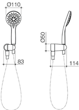
BASIS ROUND HAND SHOWER WELS 3 star rated, 9L/min BAS031C3A CHROME BAS031B3A BLACK BAS031BN3A BRUSHED NICKEL
