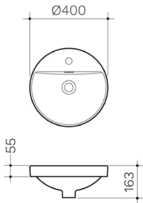
CLARK ROUND 400 SEMI RECESSED BASIN 1TH OF
