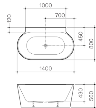
CLARK RND 1400 BTW F/S BTH NOF CL50003.WBTWN
