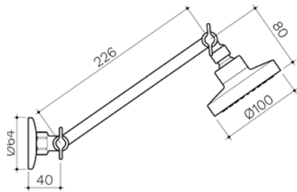
ROUND BASIC ADJUSTABLE SHOWER WELS 3 star rated, 9L/min CL10057.C3A
