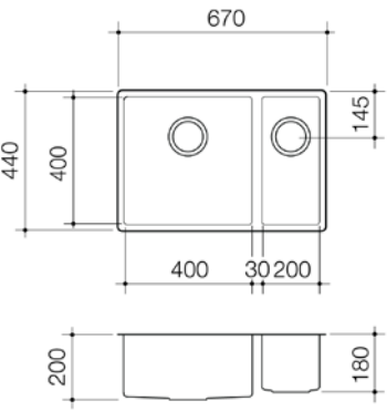
PRISM 1.5 LEFT HAND BOWL UNDERMOUNT/OVERMOUNT PPR15BLH
