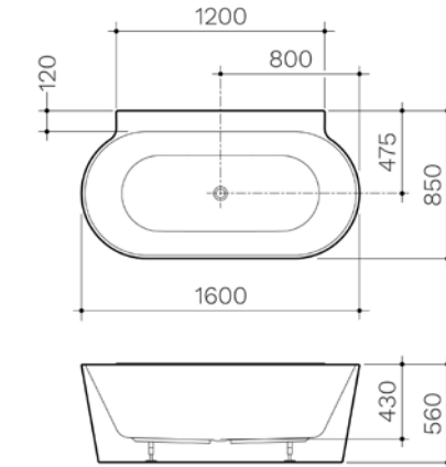
CLARK RND 1600 BTW F/S BTH NOF CL50004.WBTWN
