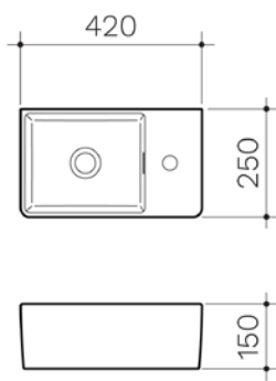
CLARK SQUARE HAND WALL BASIN 1TH OF
