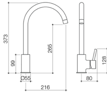
BASIS R3 SINK MIXER WELS 4 star rated, 7.5L/min BAS020C4AF CHROME BAS020B4AF BLACK BAS020BN4AF BRUSHED NICKEL
