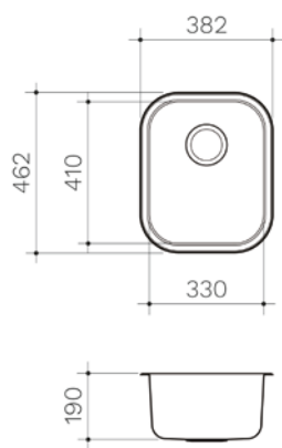
CLARK 45L SINGLE TUB 8520
