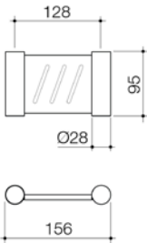
BASIS SOAP DISH BAS050C CHROME BAS050B BLACK BAS050BN BRUSHED NICKEL
