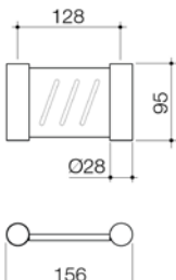
BASIS SOAP DISH BAS050C CHROME BAS050B BLACK BAS050BN BRUSHED NICKEL
