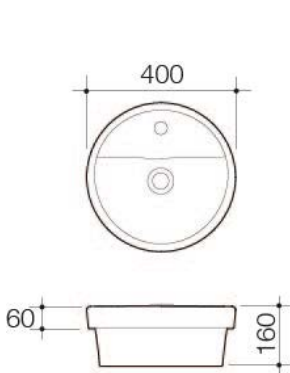
STYLUS BASIS ROUND BASIN BAS0715W
