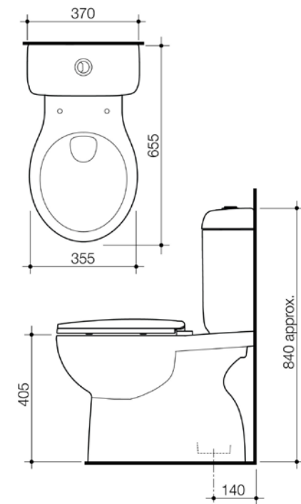
STYLUS BASIS BTW CC 4S BE SUITE
