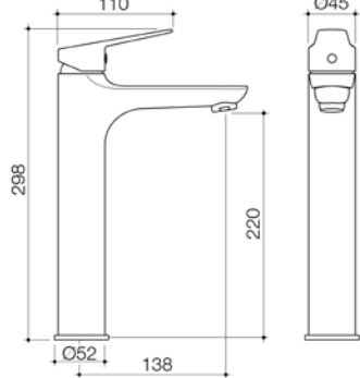
BASIS R4 TOWER BASIN MIXER BAS023C5AF CHROME BAS023B5AF BLACK BAS023BN5AF BRUSHED NICKEL
