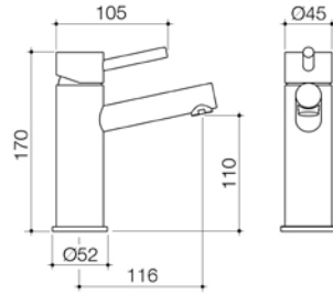
BASIS R3 BASIN MIXER WELS 5 star rated, 6L/min BAS019C5AF CHROME BAS019B5AF BLACK BAS019BN5AF BRUSHED NICKEL
