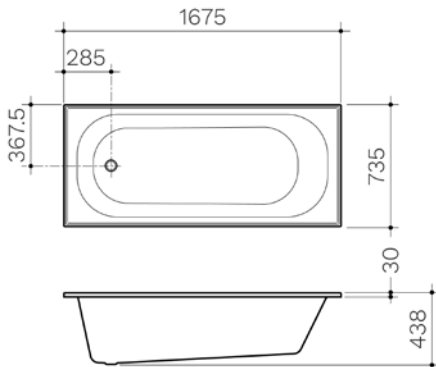
BASIS BATH 1675 4TF WHITE BB7W
