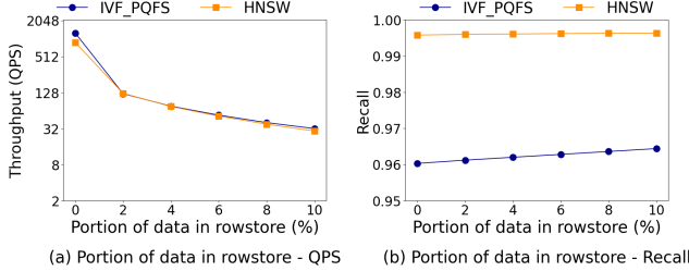
Figure 7: Varying Different Portions of Data in Rowstore of SingleStore-V
