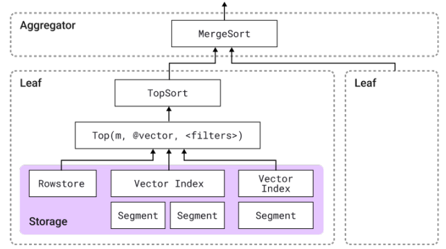
Figure 2: Vector Search in SingleStore-V
