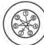
7-NUT WHEEL
