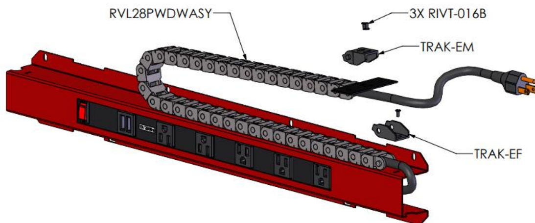
Figure 5: 4228TB Power Drawer Power Strip Detail
