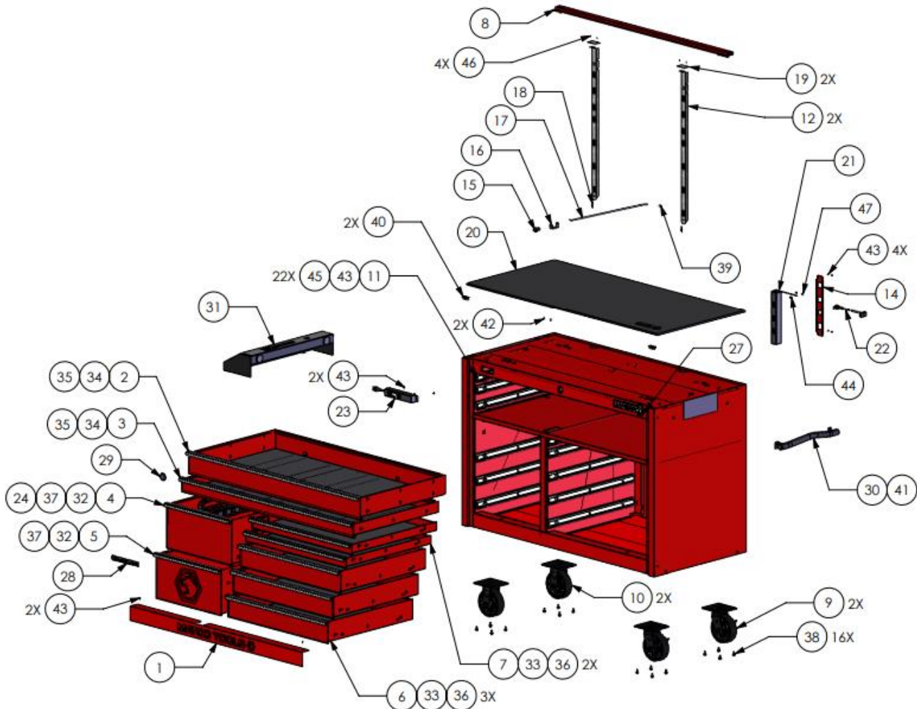
Figure 1: 4228TB Replacement Parts Exploded View
