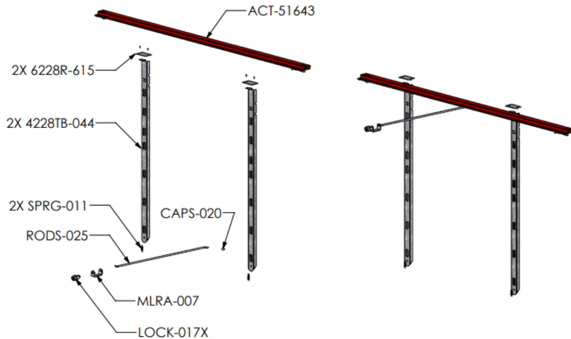
Figure 8: Replacement Parts Locking Assembly Detail for 4228TB
