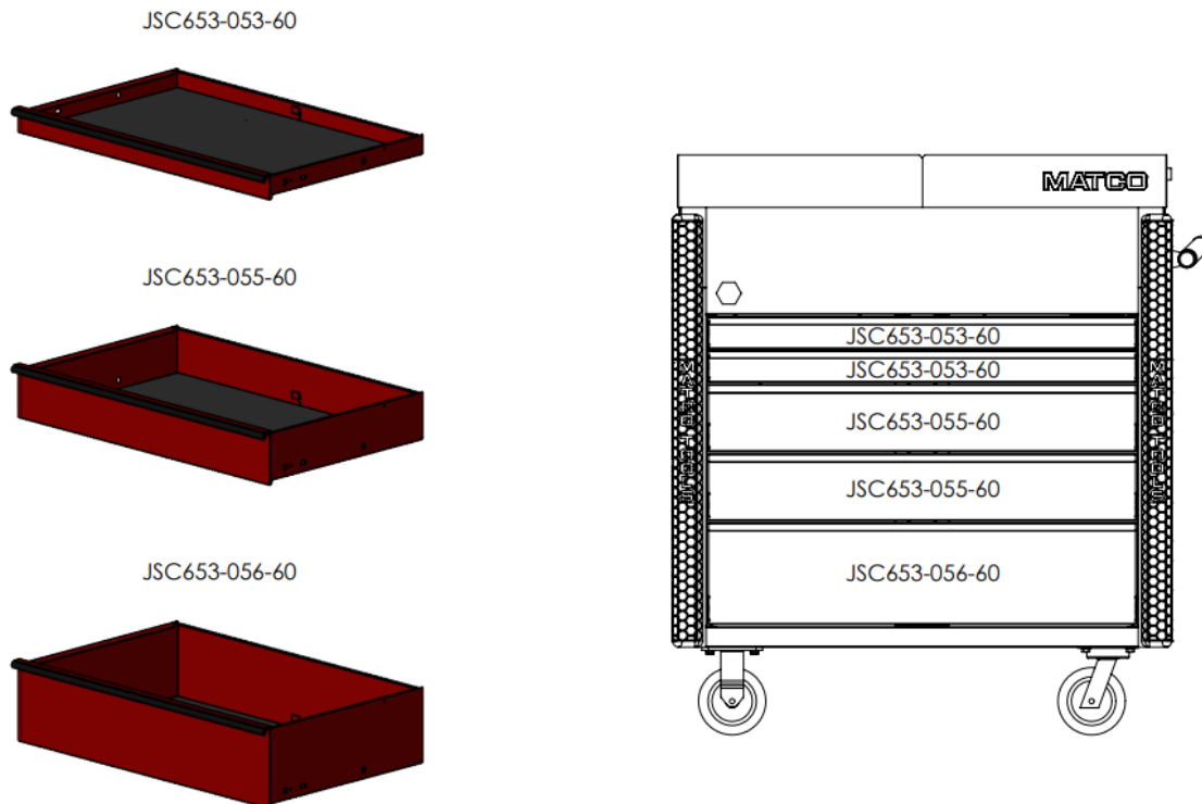
Figure 2: Drawer Configuration Detail
