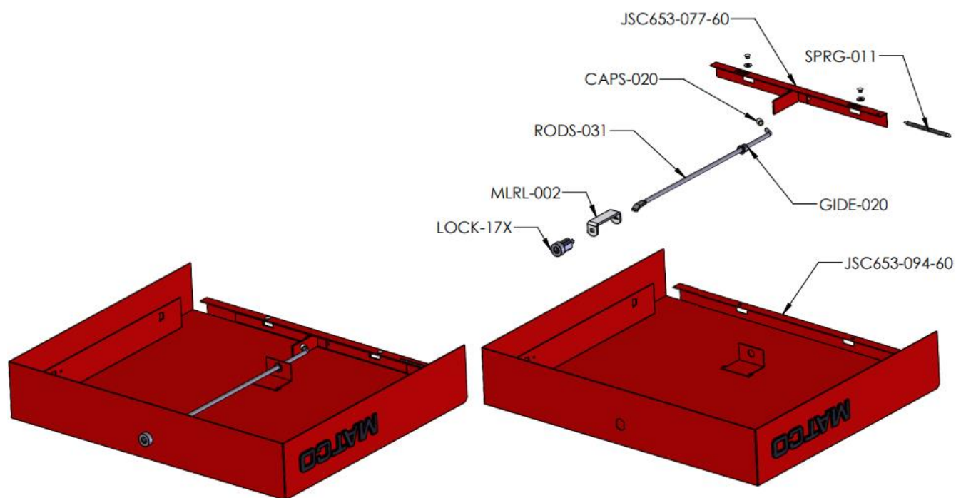
Figure 4: JSC653 Lid Locking Assembly Detail
