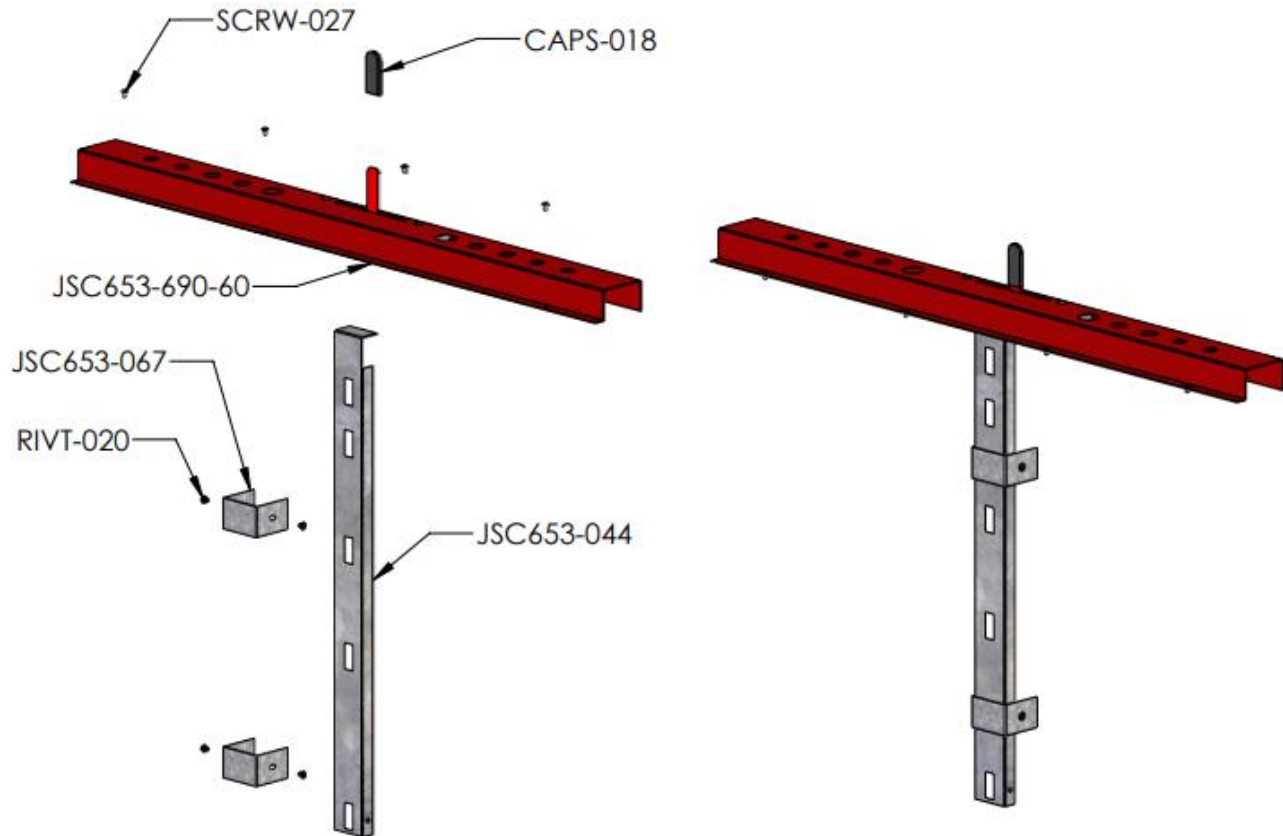
Figure 5: JSC653 Drawers Locking Assembly Detail
