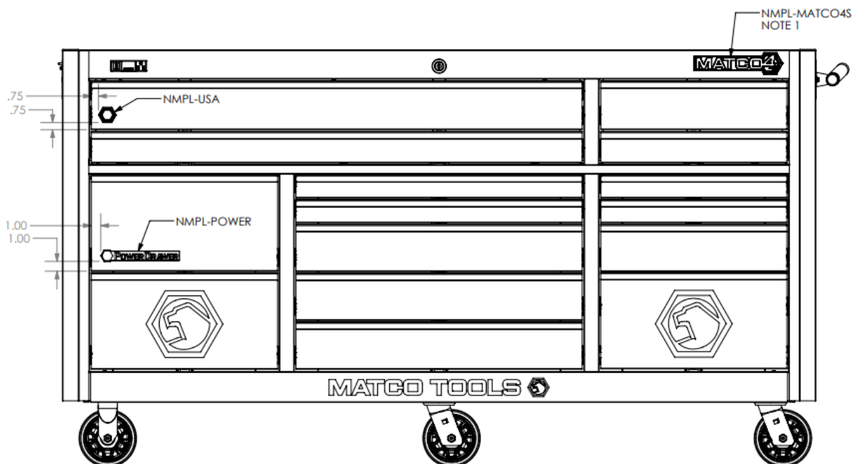
Figure 6: Emblem Positions for 4328TB
