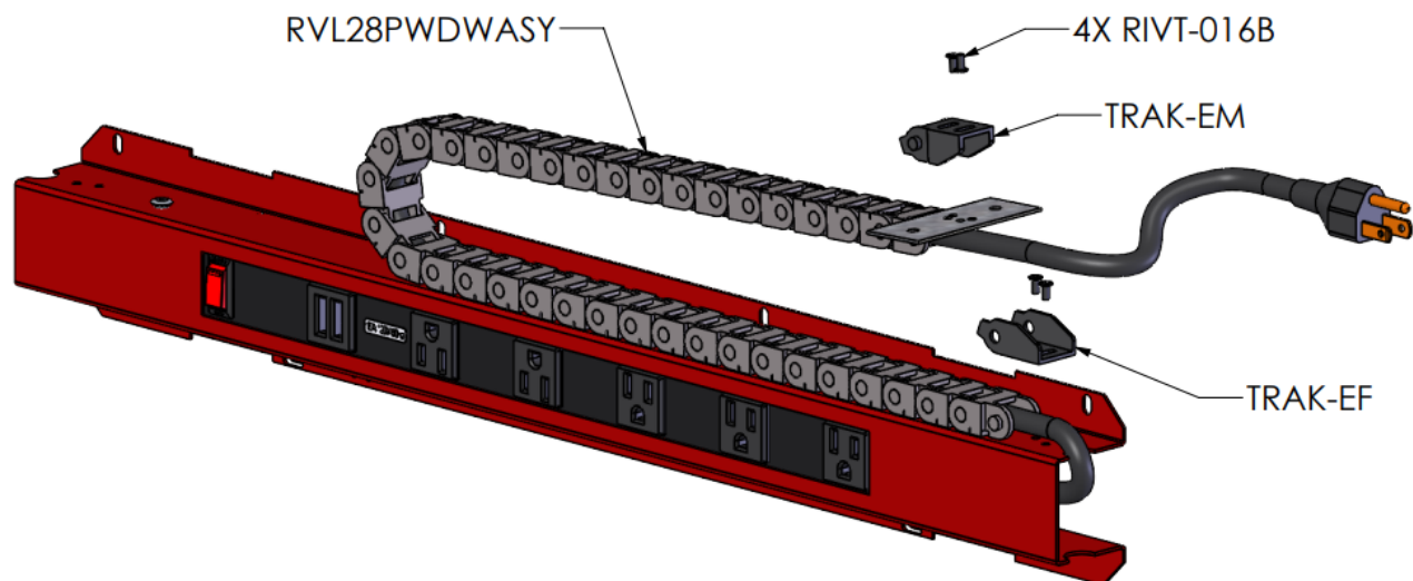
Figure 5: 4328TB Power Drawer Power Strip Detail
