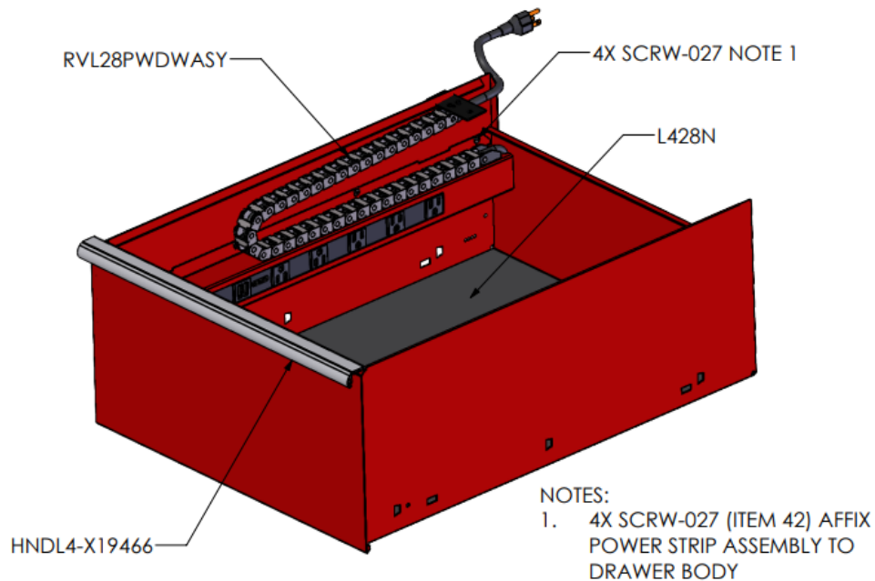
Figure 4: 42810N Power Drawer for 4328TB Detail
