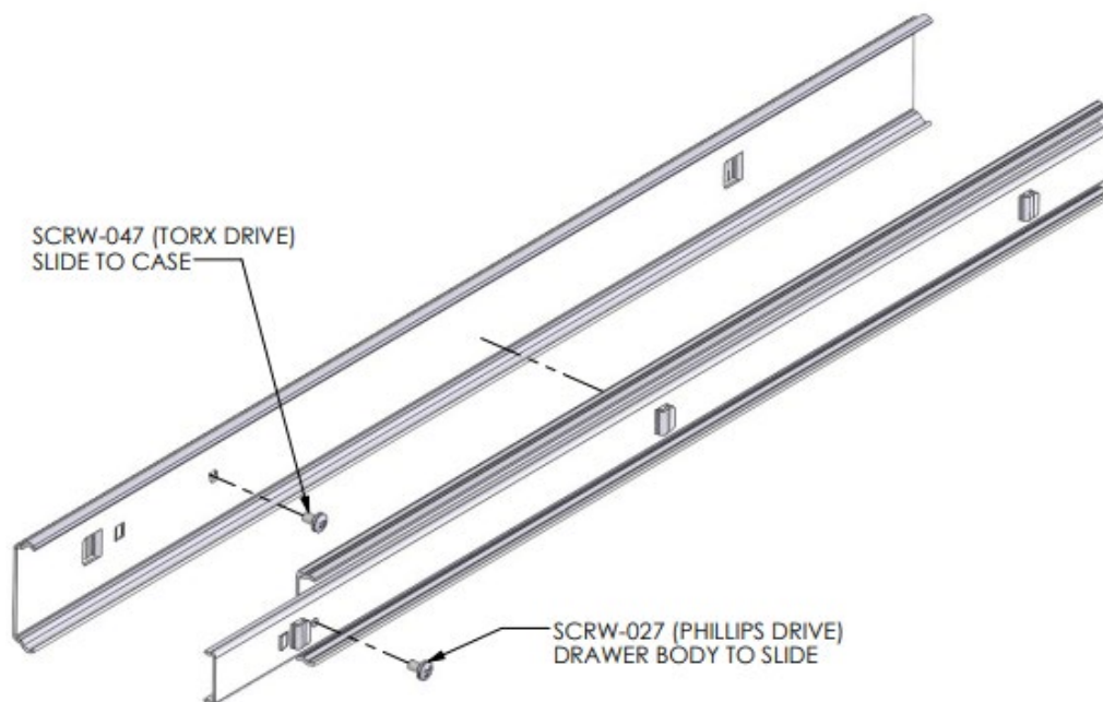
Figure 7: Slide Assembly Detail
