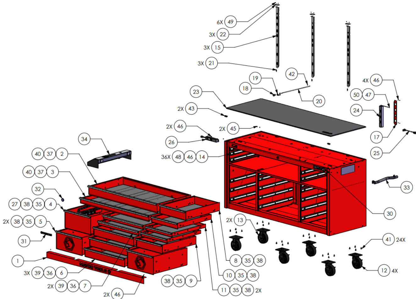
Figure 1: 4328TB Replacement Parts Exploded View
