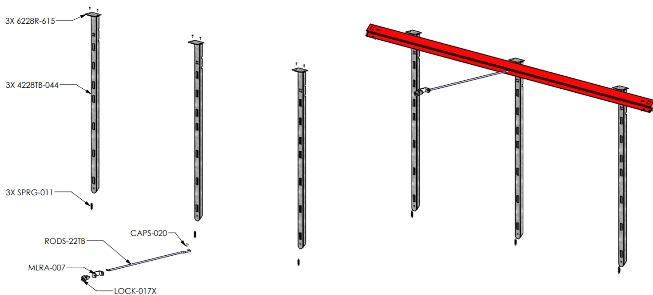
Figure 8: Replacement Parts Locking Assembly Detail for 4328TB
