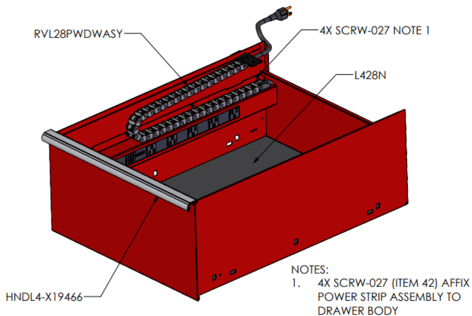
Figure 4: 42810N Power Drawer for 4228TB Detail
