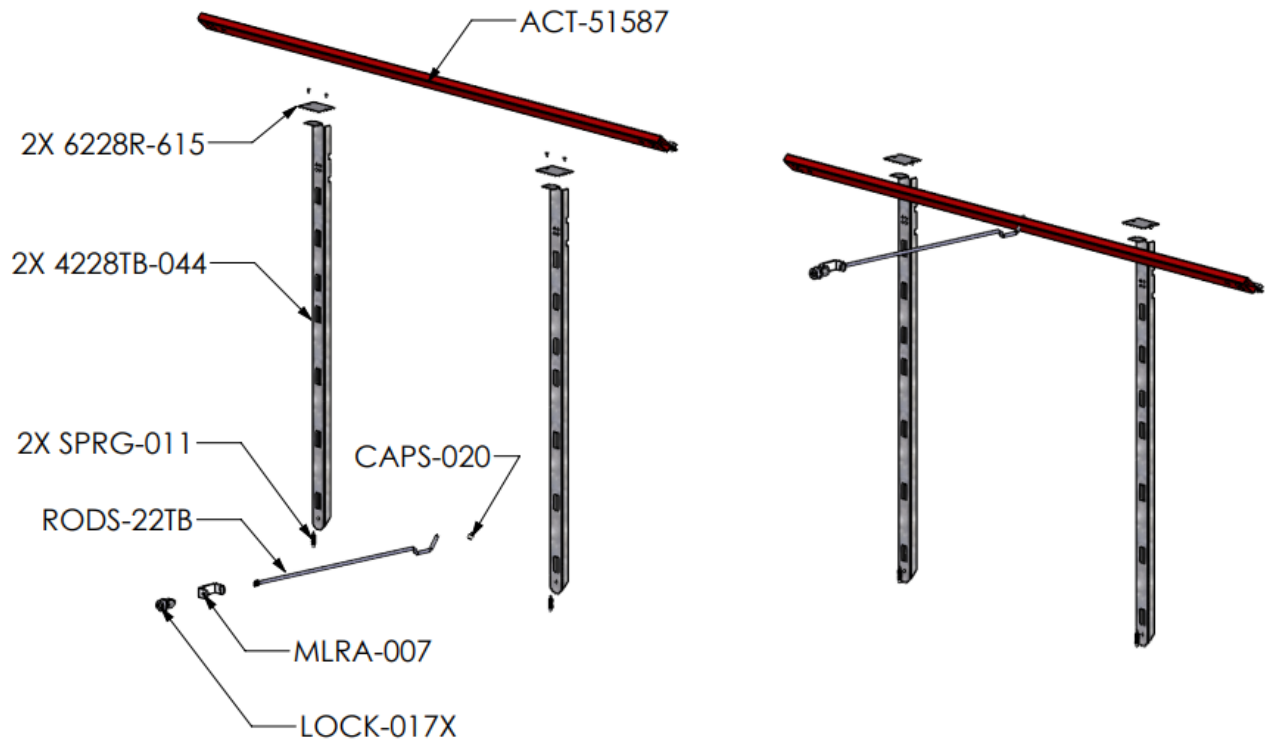
Figure 8: Replacement Parts Locking Assembly Detail for 4228TB
