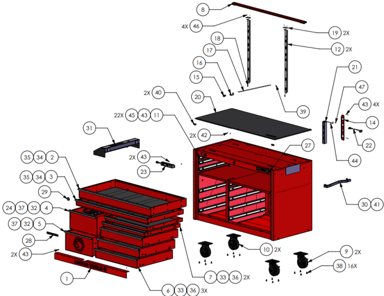
Figure 1: 4228TB Replacement Parts Exploded View
