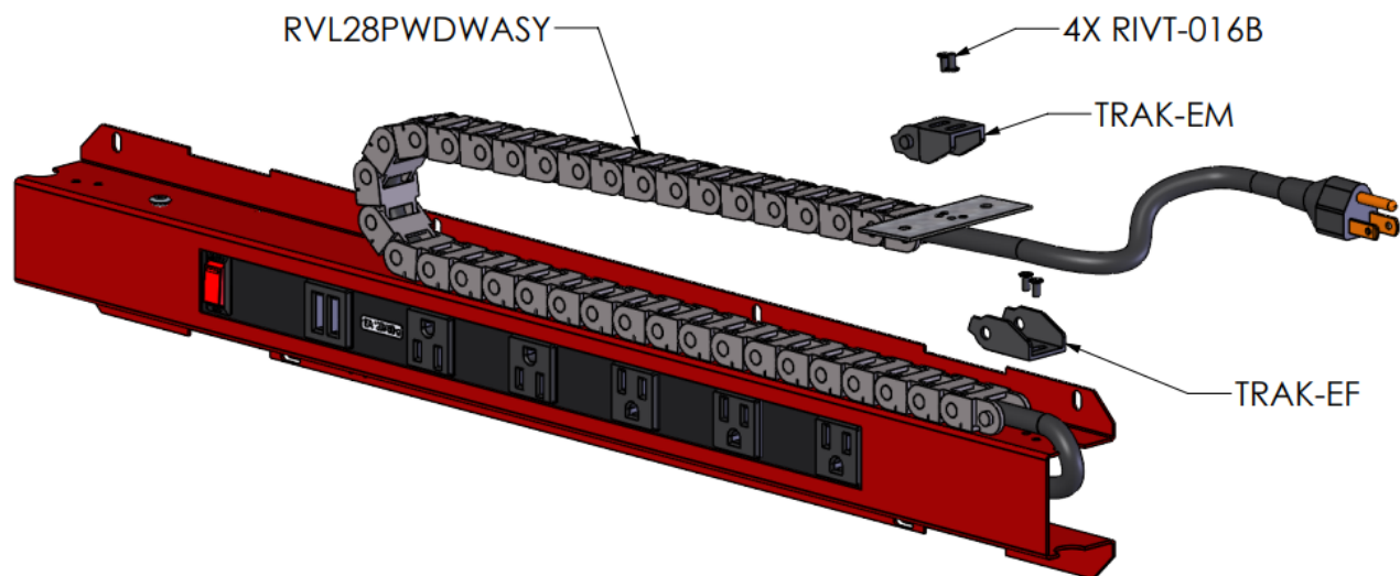
Figure 5: 4228TB Power Drawer Power Strip Detail
