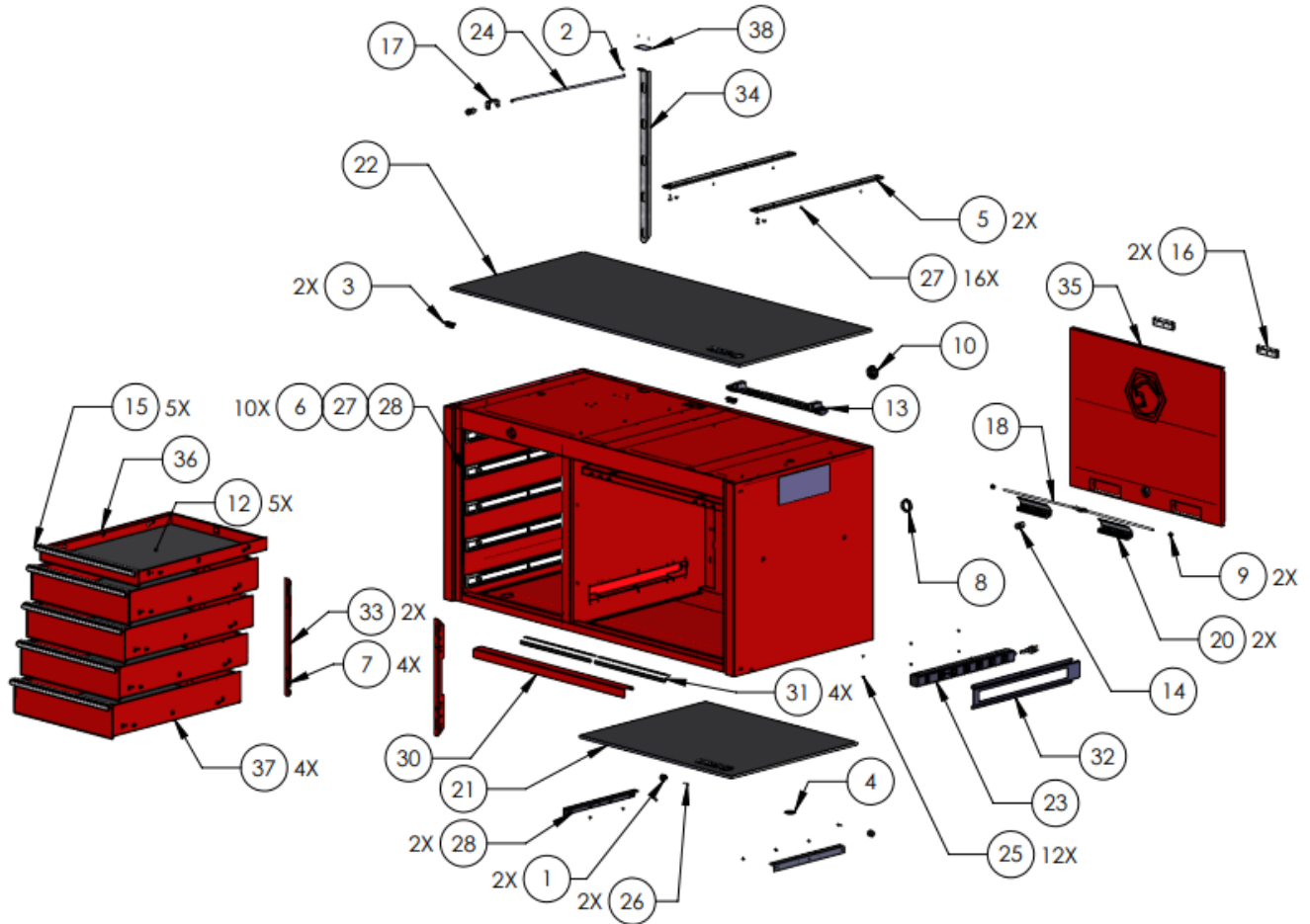
Figure 1: Replacement Part Explosion View
