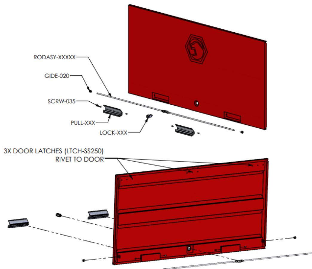
Figure 3: General Hutch Door Assembly Detail
