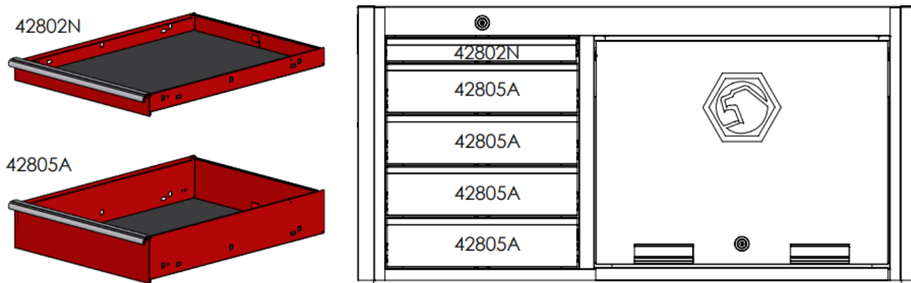
Figure 2: 4328HCA Drawer Configuration
