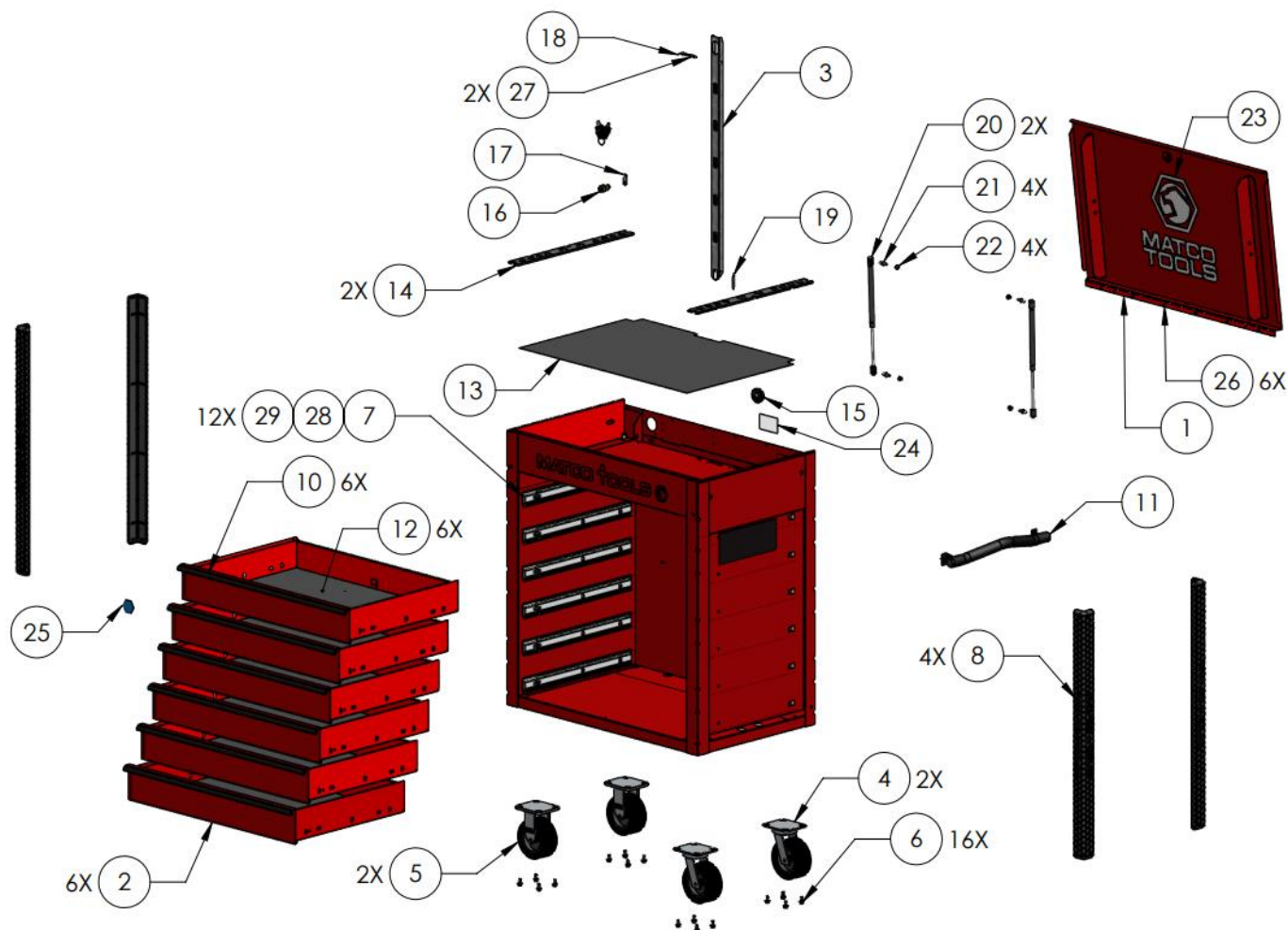
Figure 1: Replacement Part Explosion View
