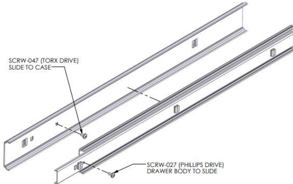
Figure 3: Slide Assembly Detail
