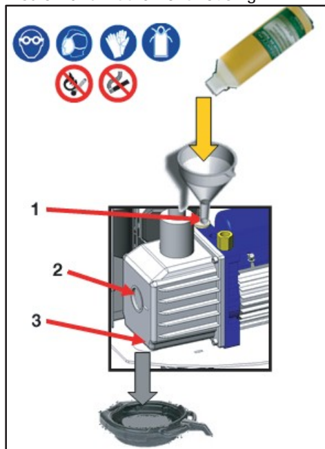
Fig. 27: Changing vacuum pump oil
