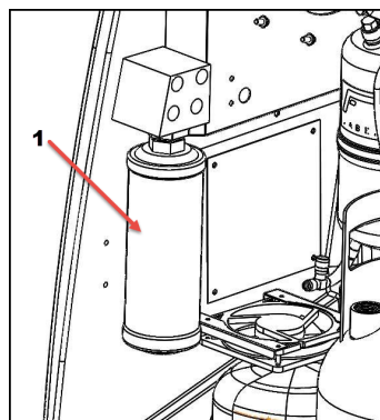
Fig. 28: Changing filter dryer
