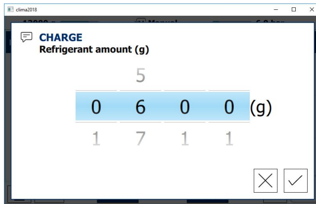
Fig. 18: Charge amount adjustment
