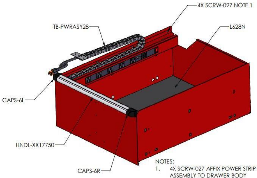
Figure 5: 6S TB Power Drawer Power Strip Detail
