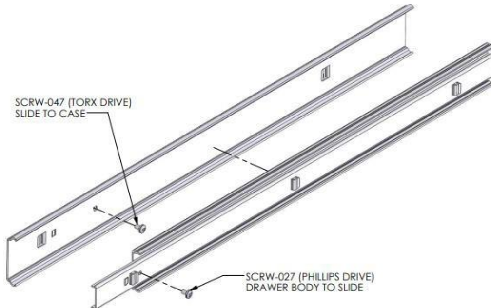
Figure 7: Slide Assembly Detail
