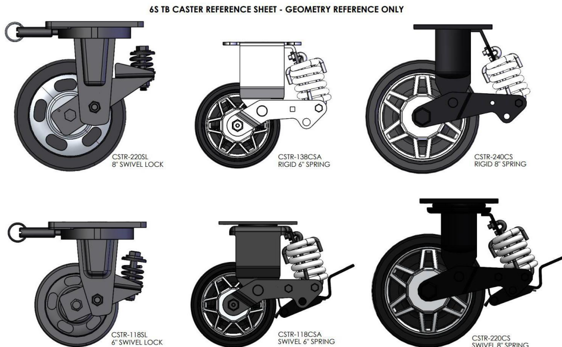
Figure 10: 6S TB Caster Option Reference Detail
