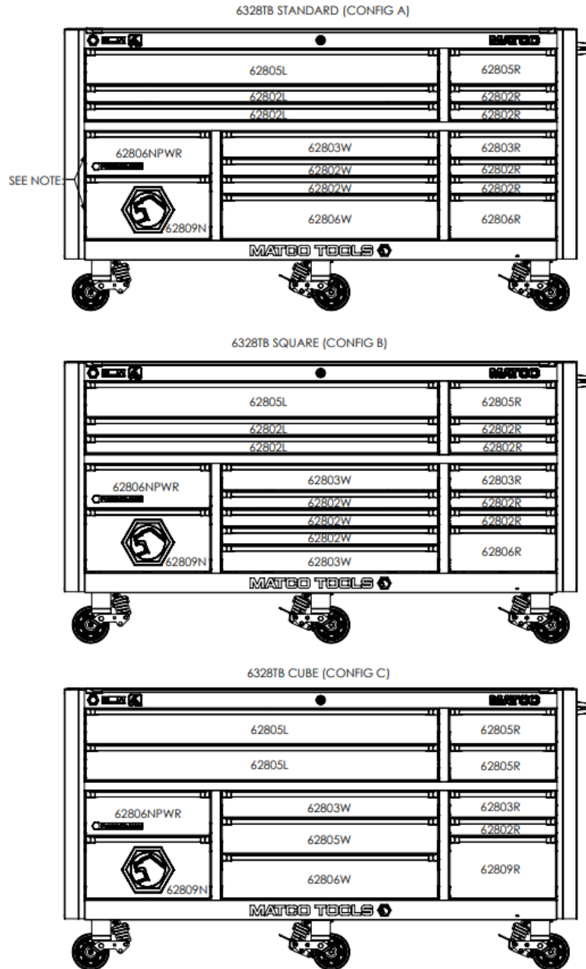
Figure 2: 6328TB Drawer Configurations (A, B, C)
