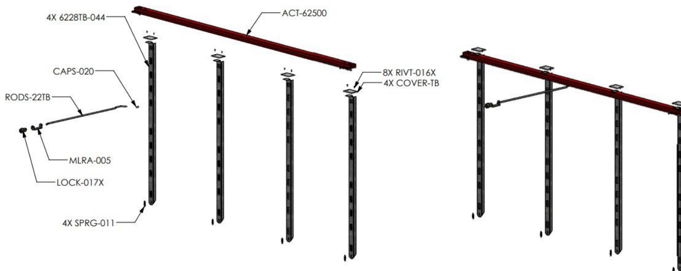
Figure 9: Lightbar Kit (TFLA-XXYYYYY) Replacement Part Detail
