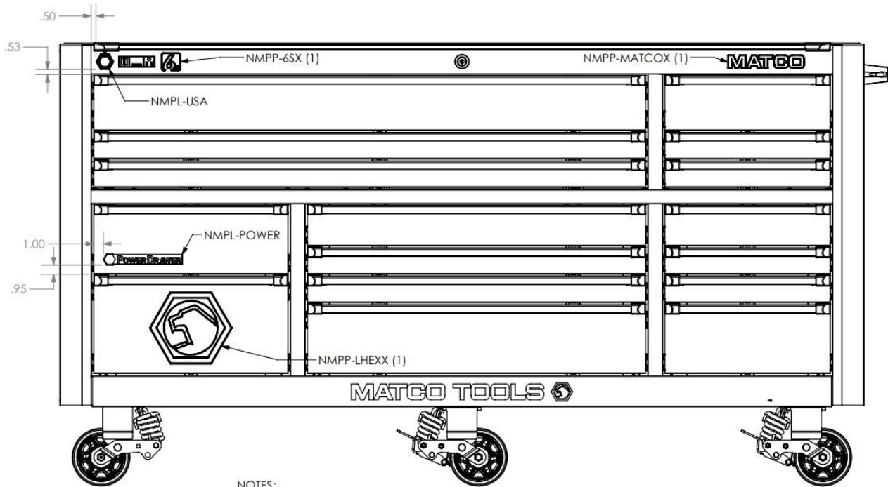
Figure 6: Emblem Positions for 6328TB
