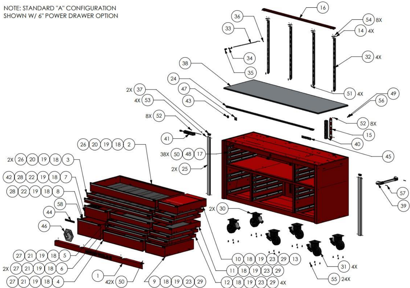
Figure 1: 6328TB W/ Standard Options Replacement Parts Exploded View
