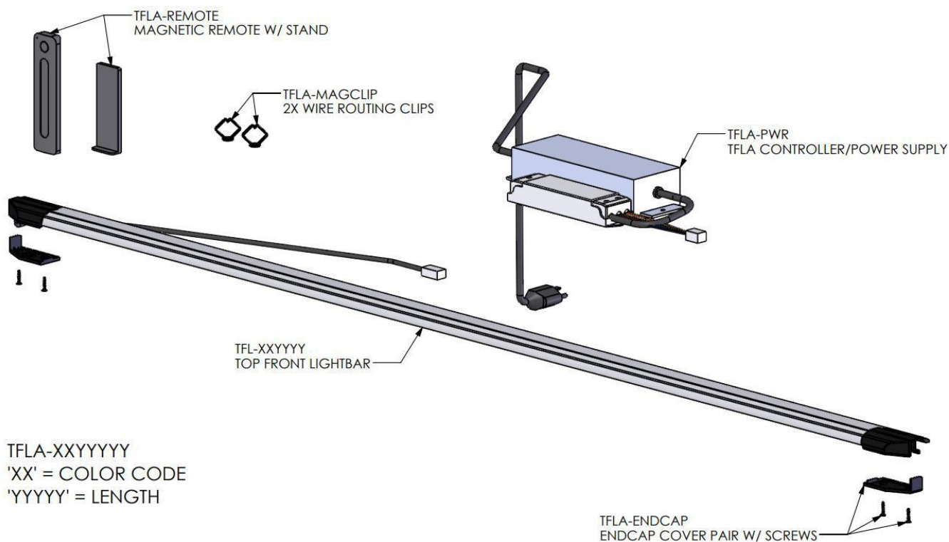
Figure 9: Lightbar Kit (TFLA-XXYYYYY) Replacement Part Detail
