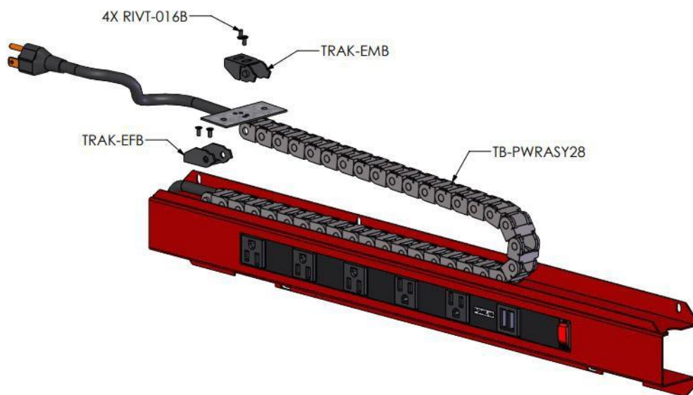
Figure 5: 6S TB Power Drawer Power Strip Detail
