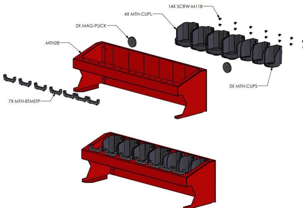
Figure 11: MTH28ASY Tool Holster Reference Detail
