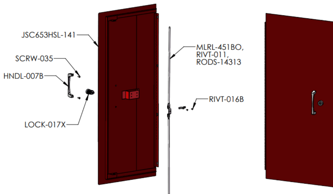
Figure 2: JSC653 Door Assembly Detail
