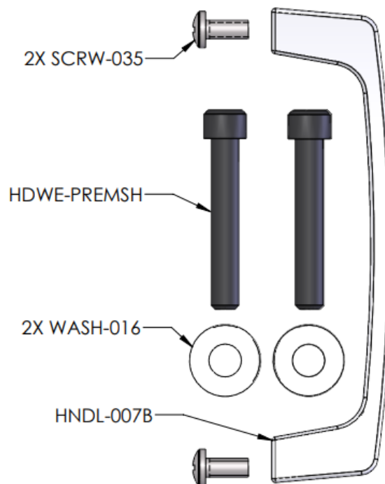
Figure 3: Hardware Included Detail
