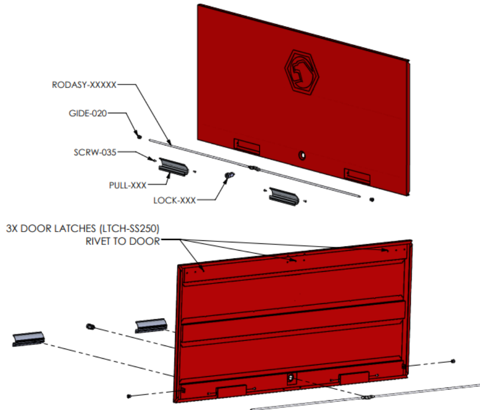
Figure 2: General Hutch Door Assembly Detail
