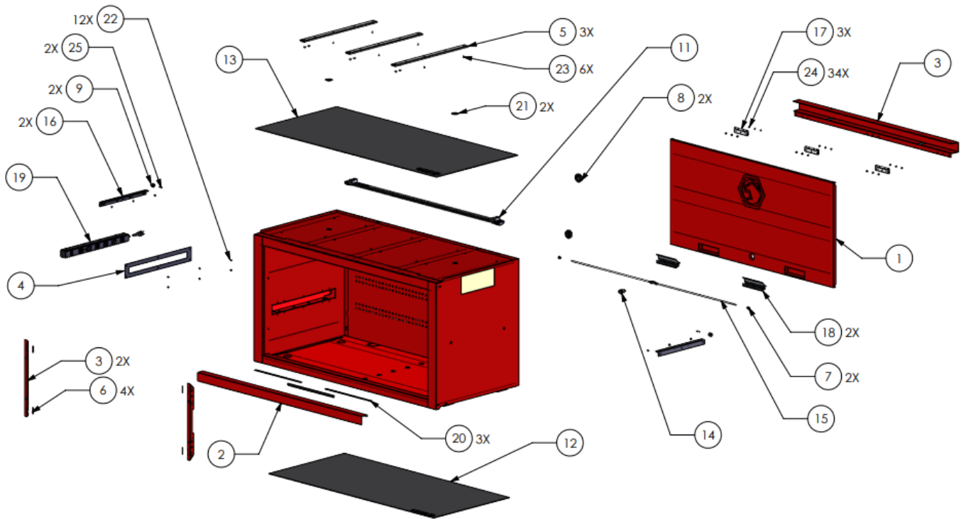
Figure 1: Replacement Part Explosion View
