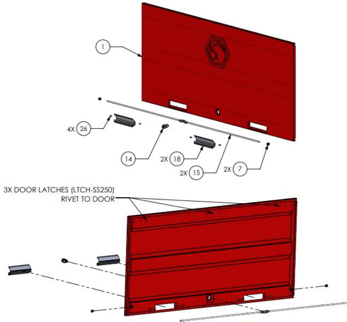
Figure 2: Door Assembly Detail
