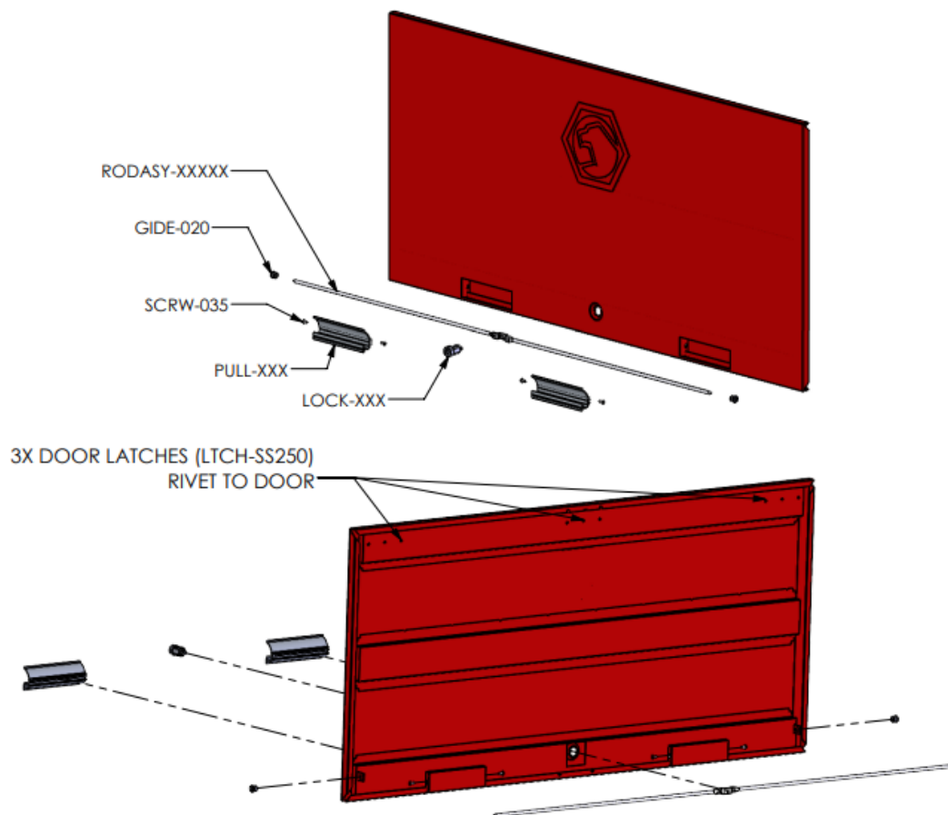
Figure 2: Door Assembly Detail
