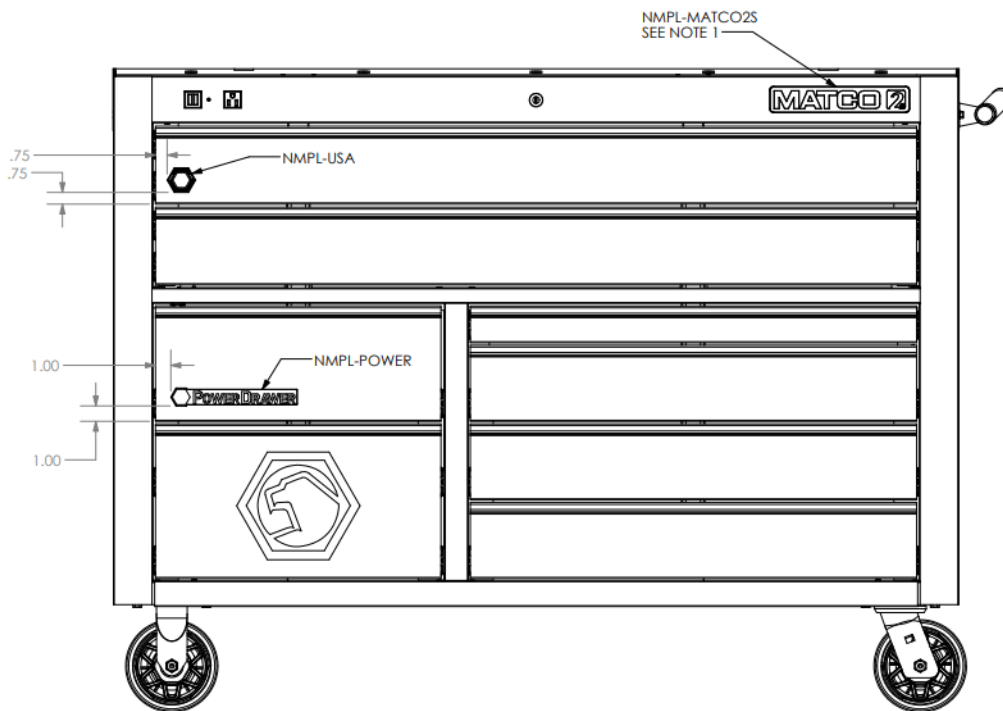
Figure 6: Emblem Positions for 2225TB
