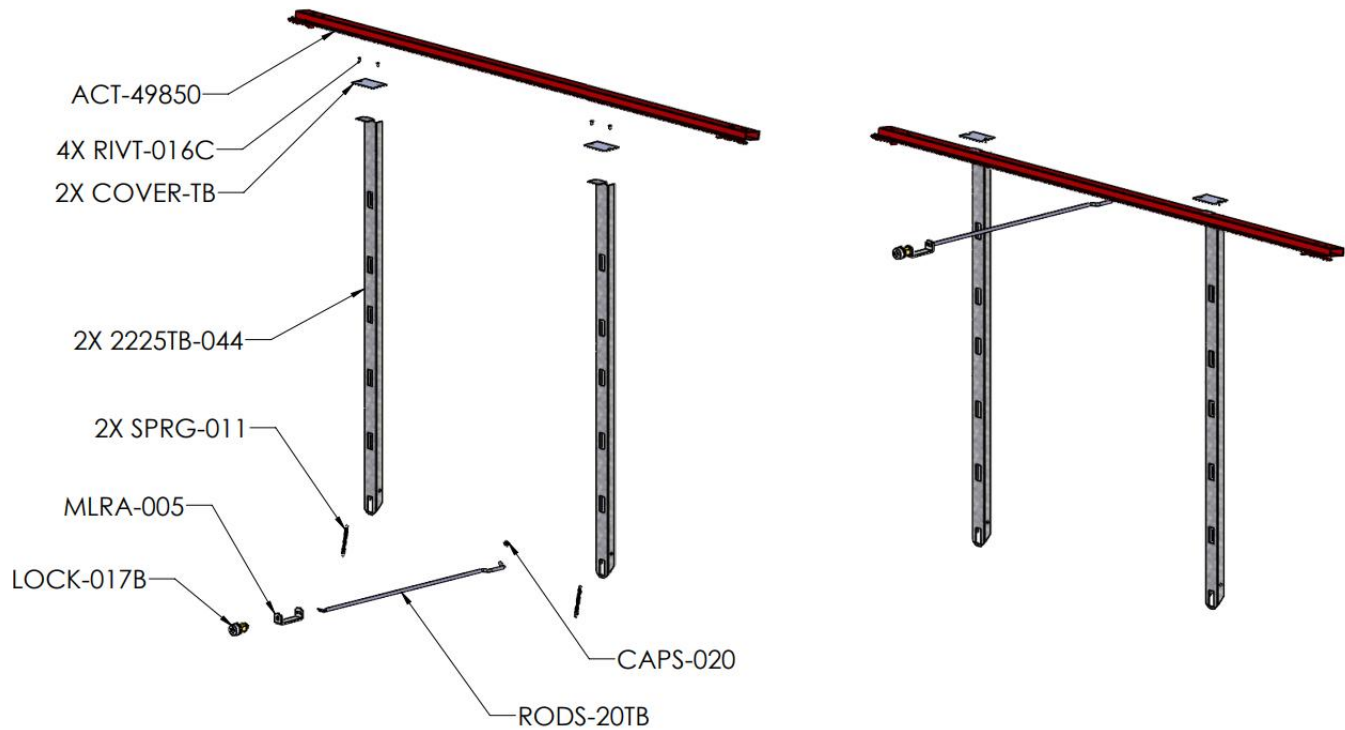
Figure 8: Replacement Parts Locking Assembly Detail for 2225TB
