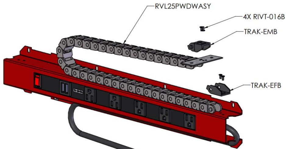
Figure 5: Power Drawer Power Strip Detail
