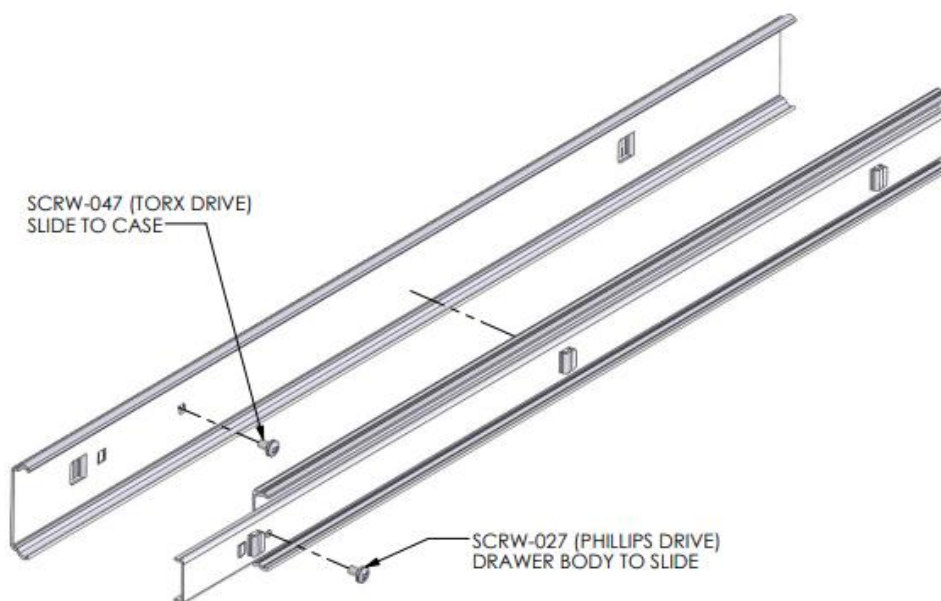
Figure 7: Slide Set (CHRN-622D) Assembly Detail for 2225TB
