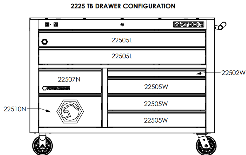
Figure 2: 2225TB Drawer Configuration
