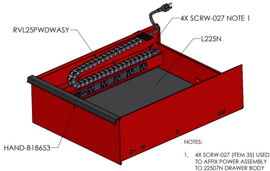
Figure 5: Power Drawer Power Strip Detail
