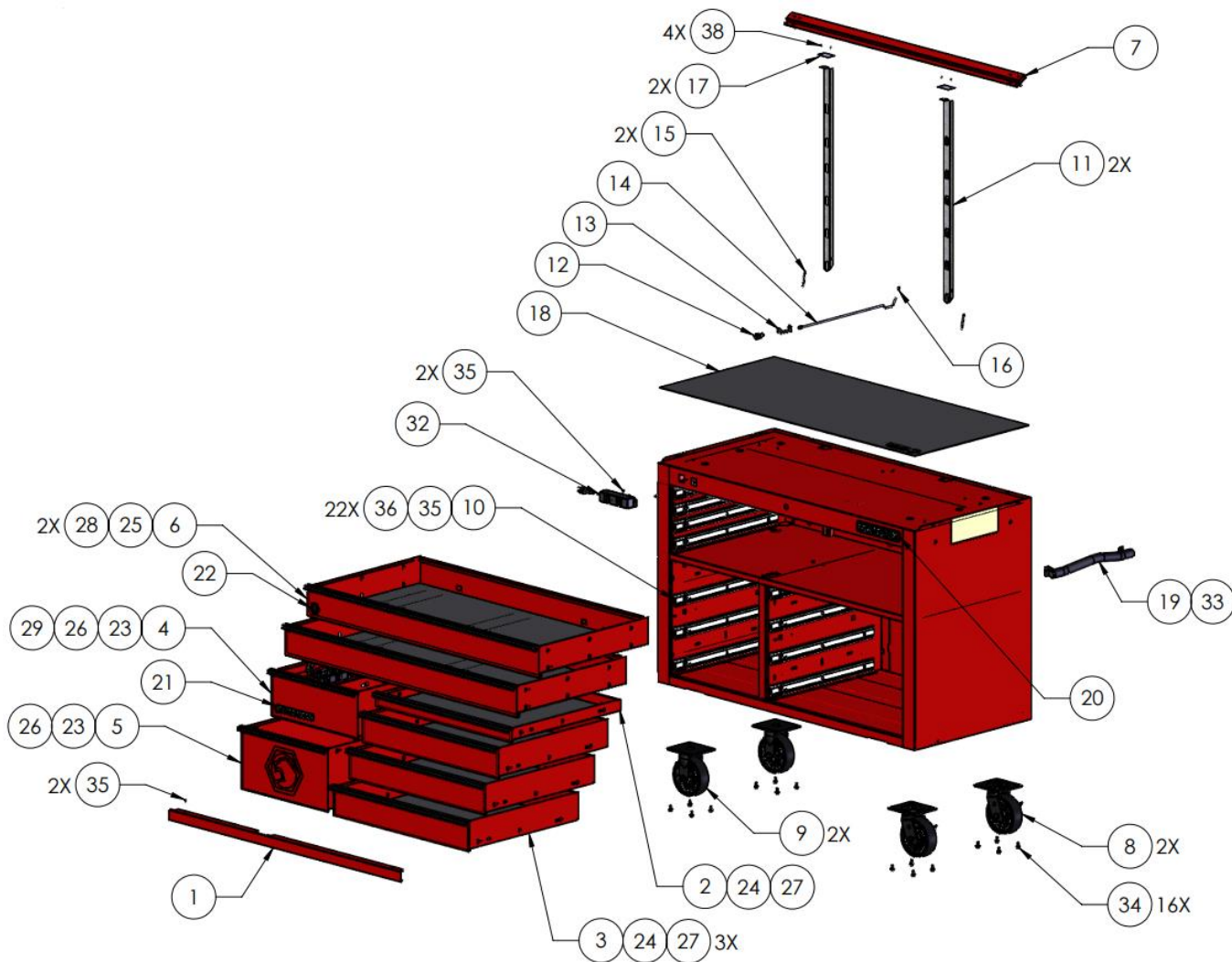
Figure 1: 2225TB Replacement Parts Exploded View
