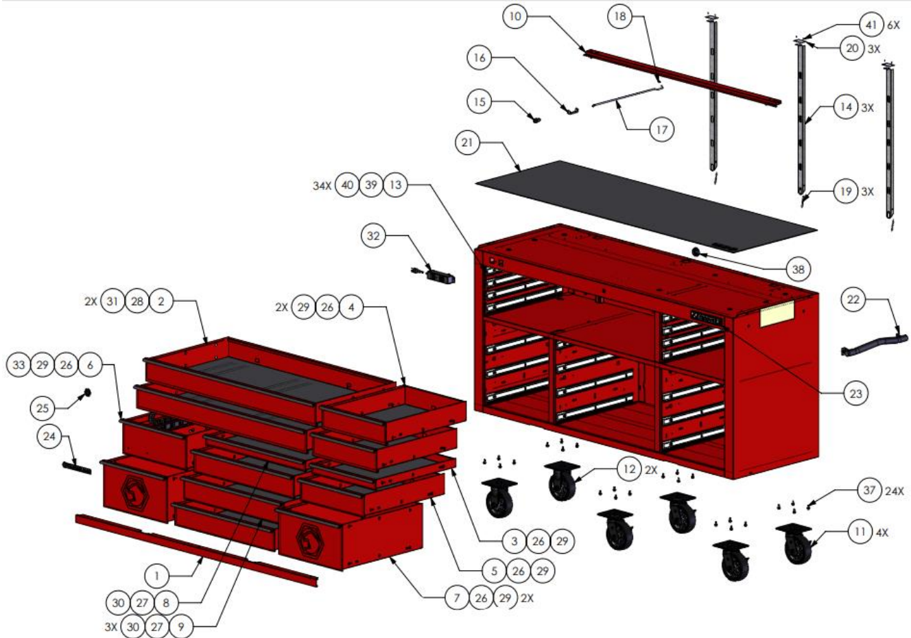
Figure 1: 2325TB Replacement Parts Exploded View
