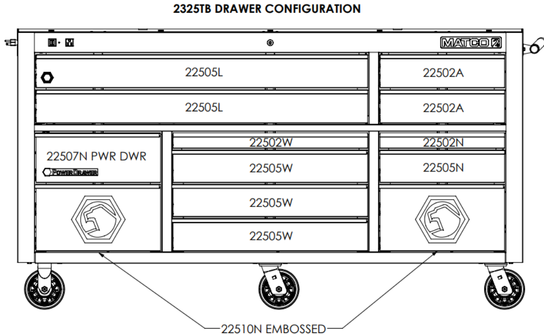
Figure 2: 2325TB Drawer Configuration
