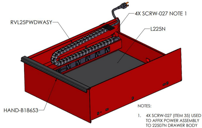
Figure 5: Power Drawer Power Strip Detail
