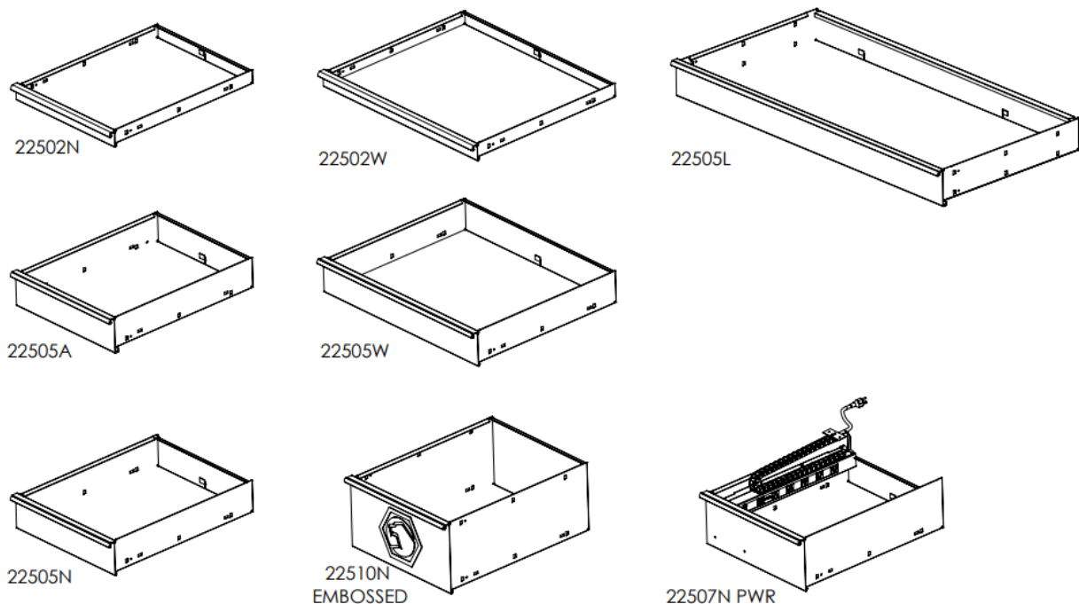
Figure 3 - Table 1: 2325TB Drawer Variants
