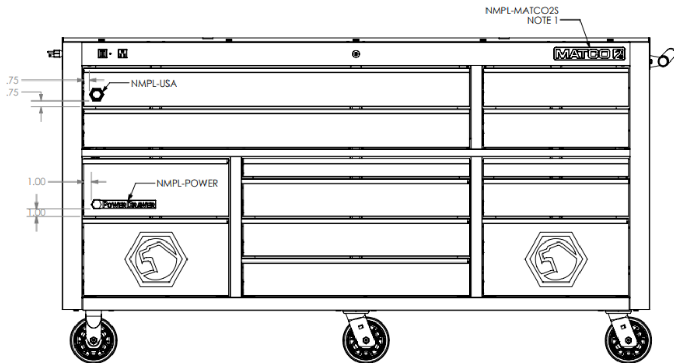
Figure 6: Emblem Positions for 2325TB
