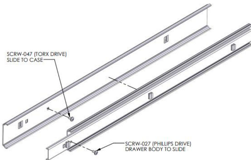
Figure 7: Slide Assembly Detail
