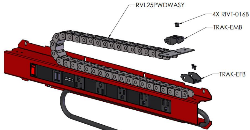
Figure 5: Power Drawer Power Strip Detail
