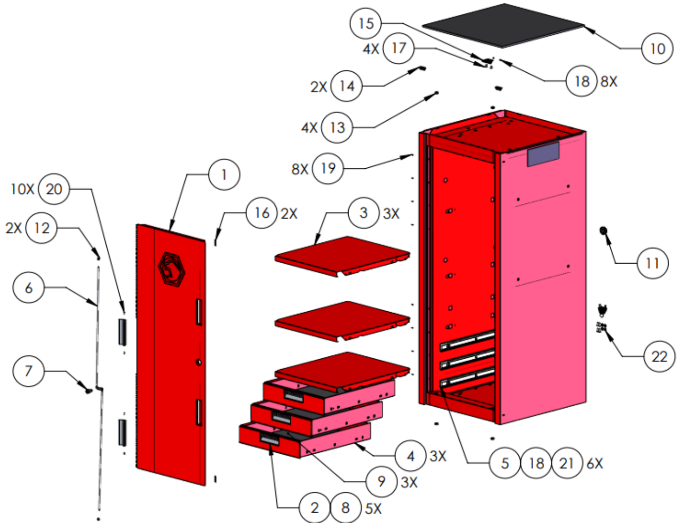
Figure 1: Replacement Part Explosion View
