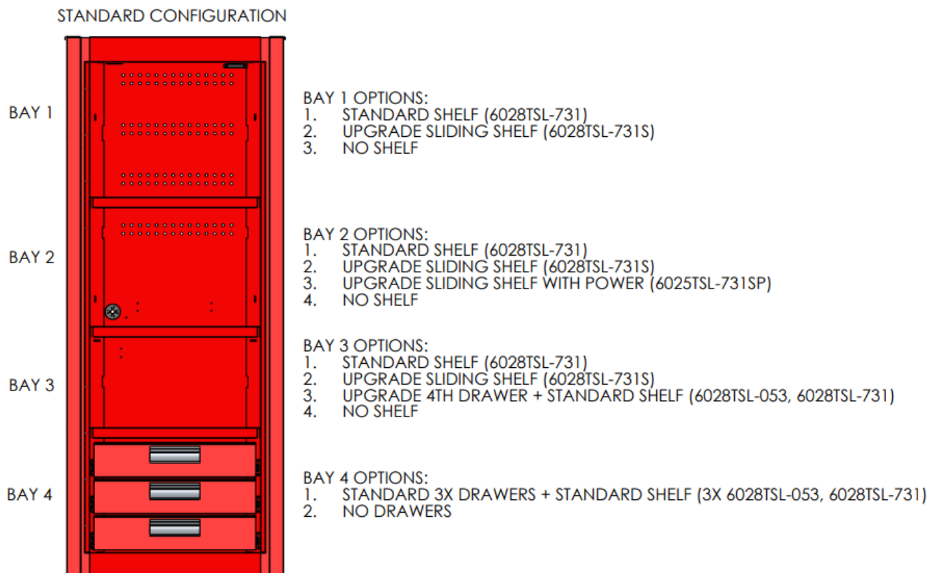
Figure 2: Upgrade Configuration Detail
