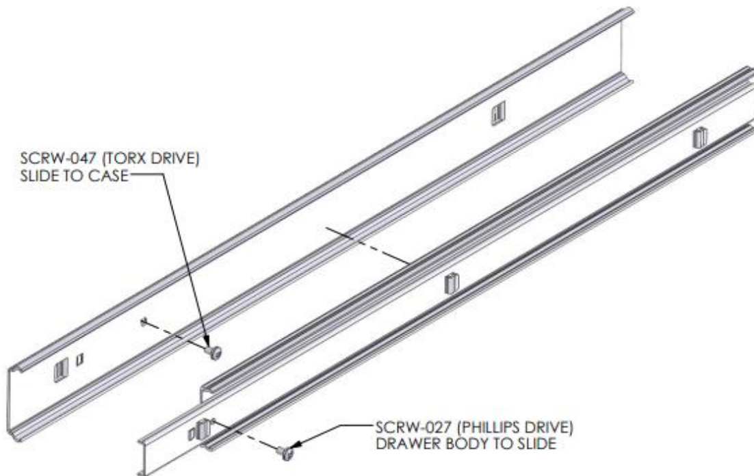
Figure 3: Slide Assembly Detail
