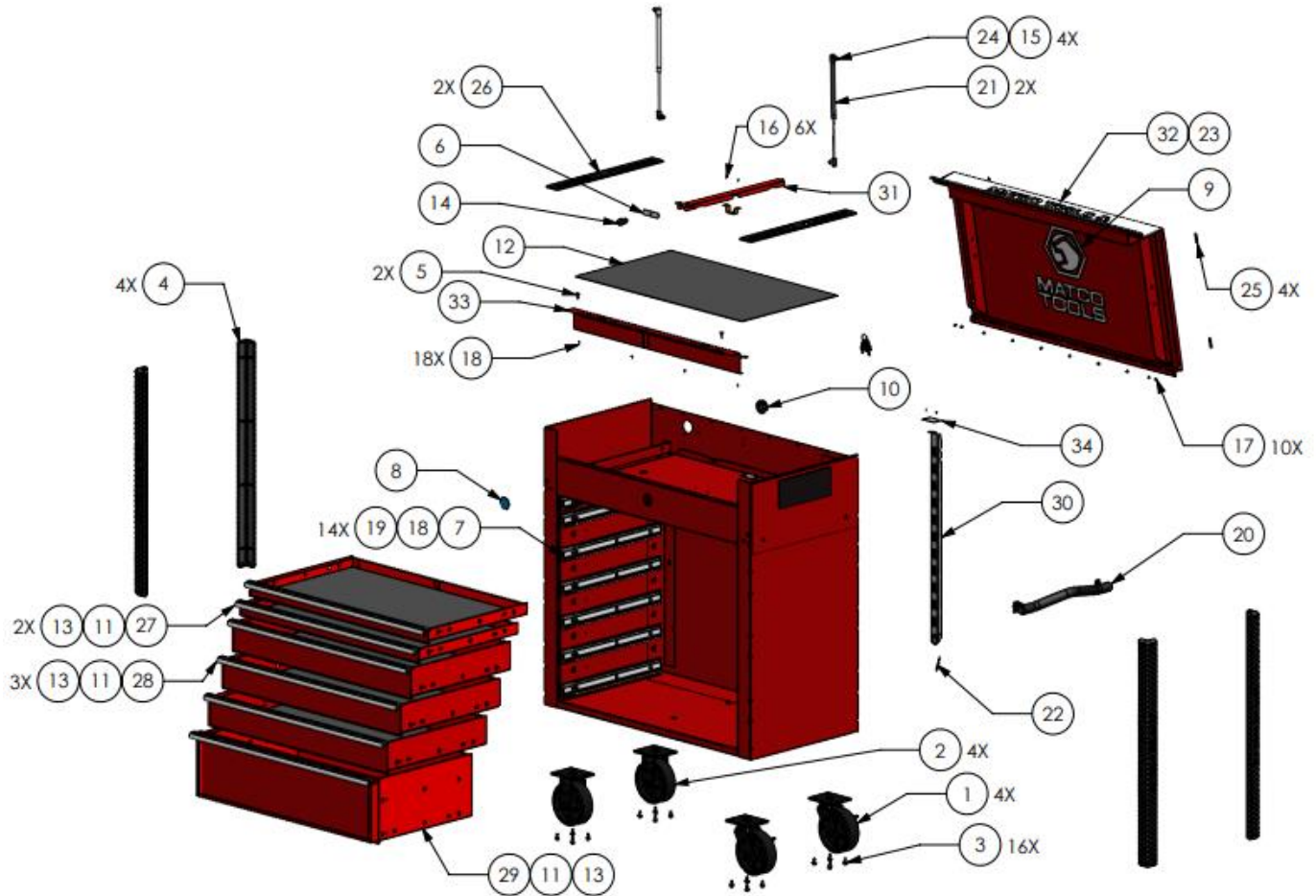
Figure 1: Standard Drawer Configuration (A) Replacement Part Explosion View
