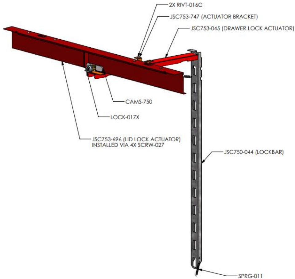
Figure 4: JSC7XX Locking Assembly Detail
