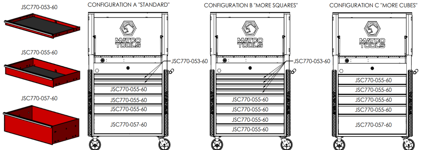
Figure 2: Drawer Configurations A, B and C Detail
