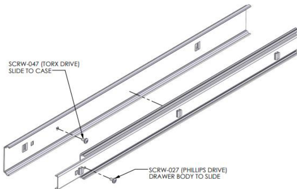
Figure 3: Slide Assembly Detail
