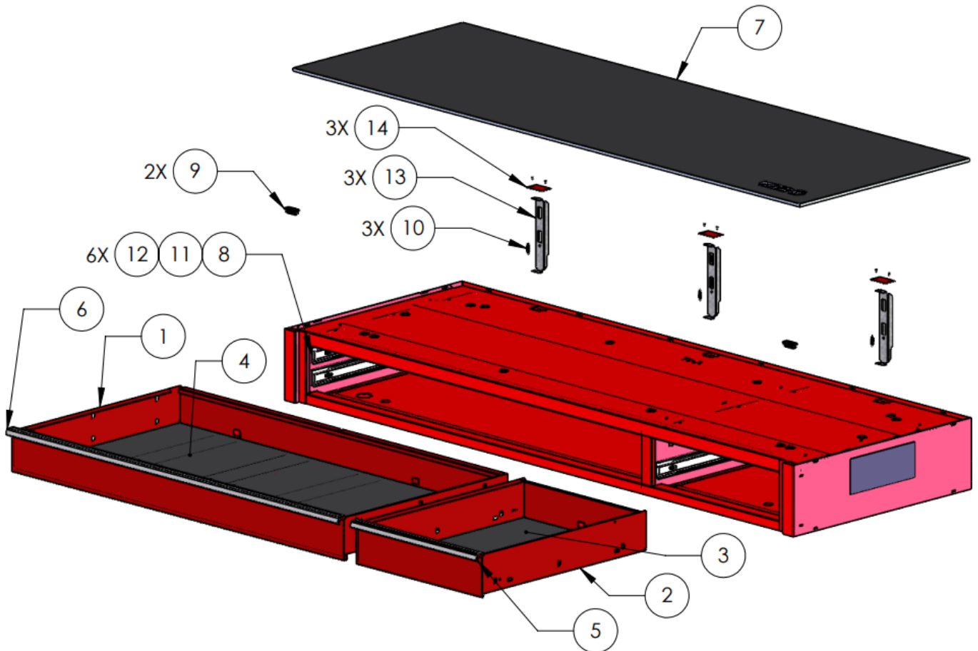
Figure 1: Replacement Part Explosion View
