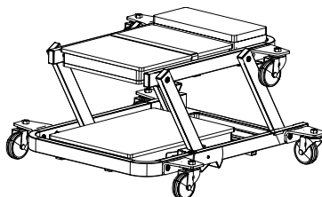
Figure 2- Seat configuration
