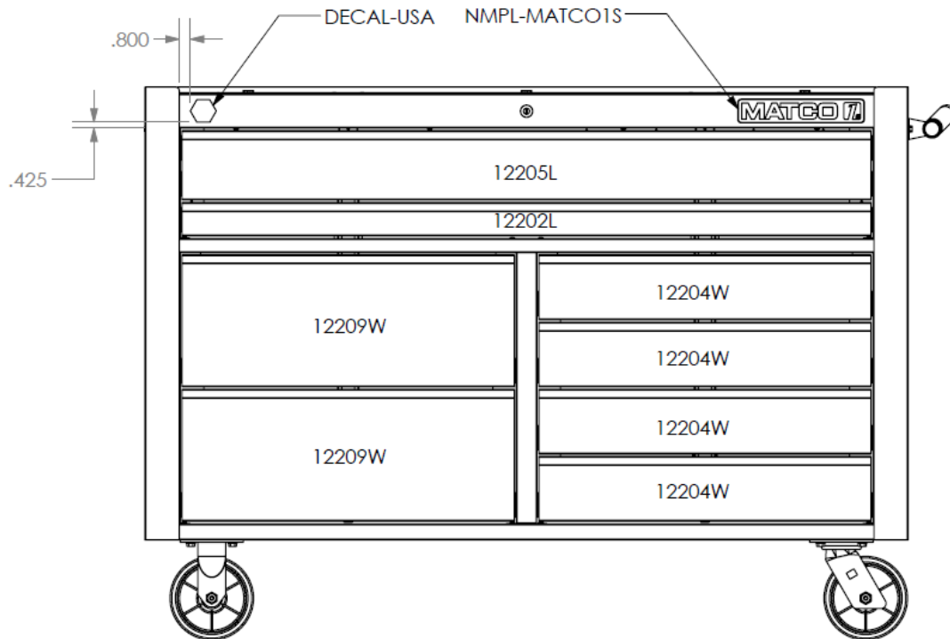
Figure 2: 1222TB Drawer Configuration & Emblem Positions
