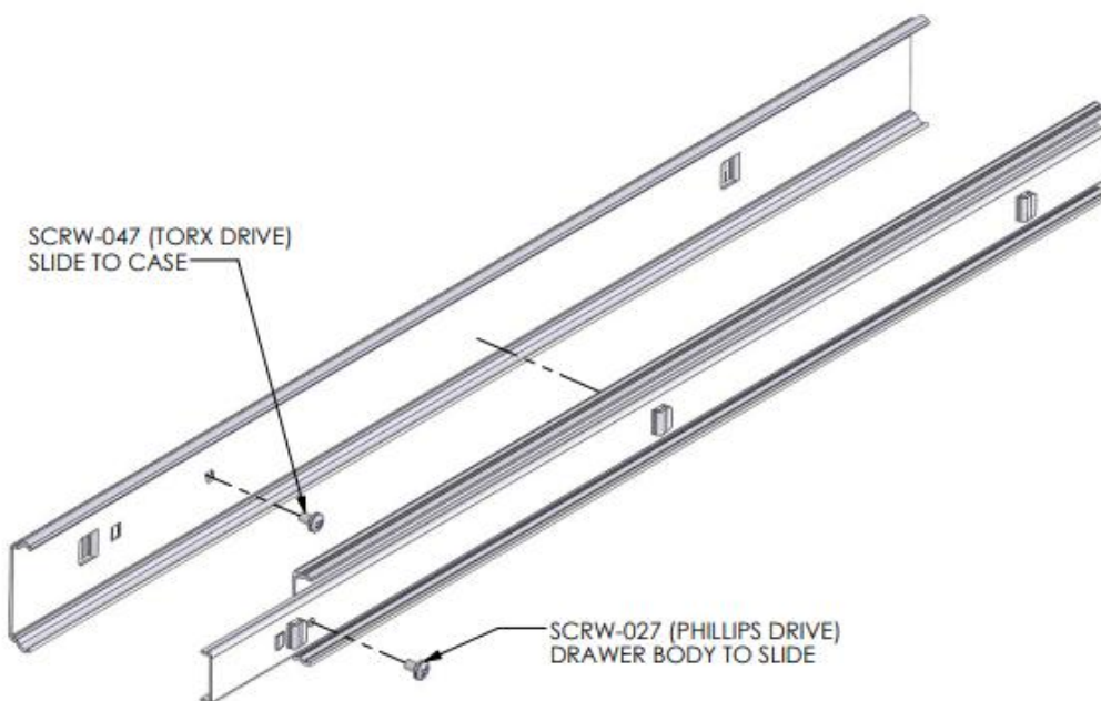
Figure 6: Slide Assembly Detail
