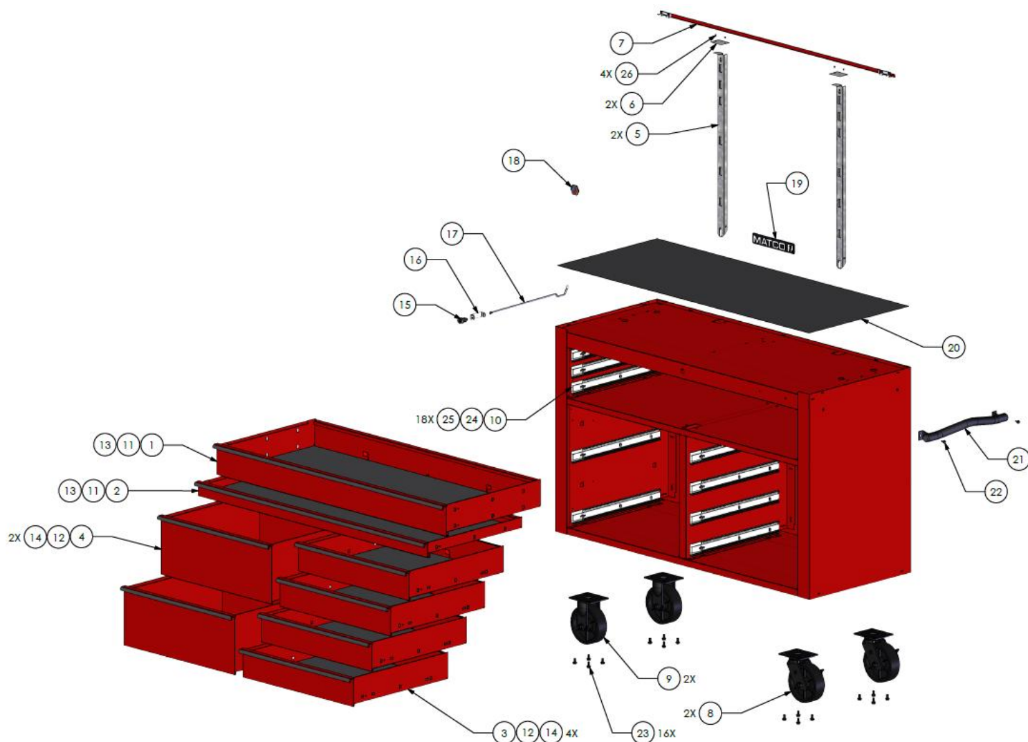
Figure 1: Replacement Parts Exploded View
