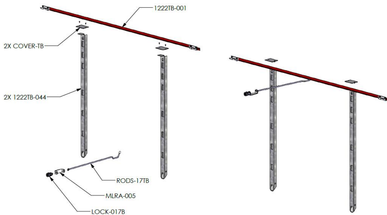
Figure 5: Locking Assembly Detail for 1222TB
