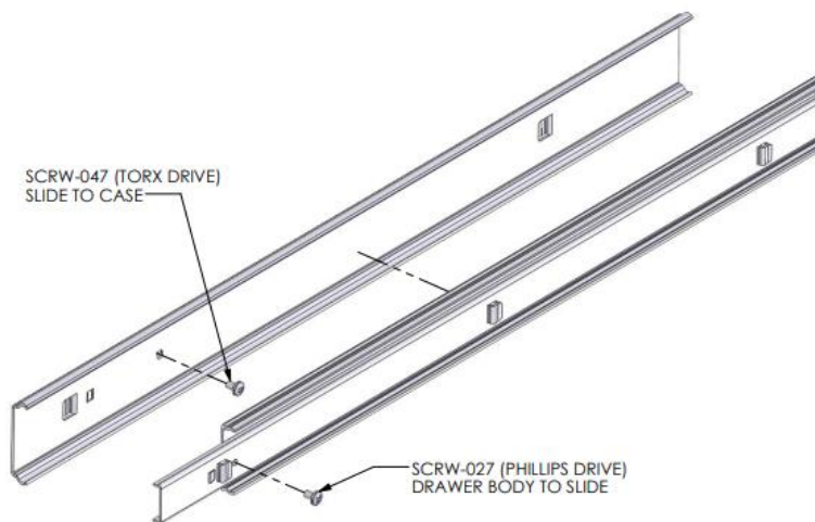
Figure 5: Slide Assembly Detail
