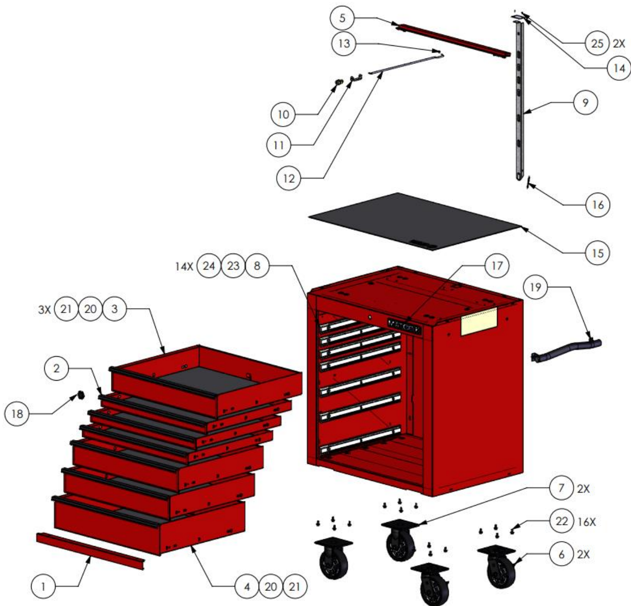
Figure 1: 2125TB Replacement Parts Exploded View
