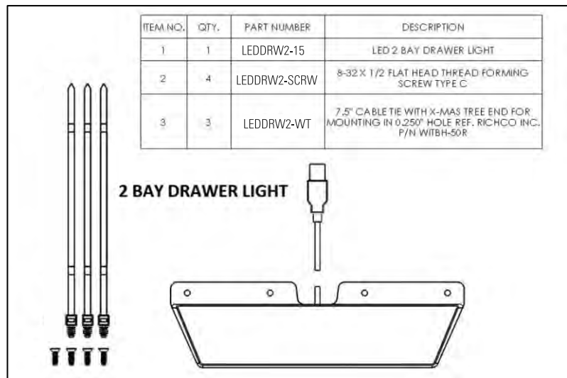
Figure 1 - Two bay toolbox drawer light kit
