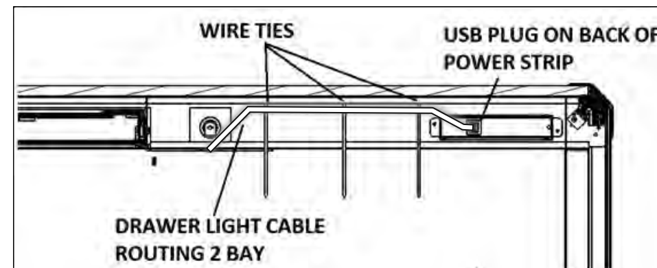
Figure 4 - Reverse view front of toolbox showing wire tie and USB locations
