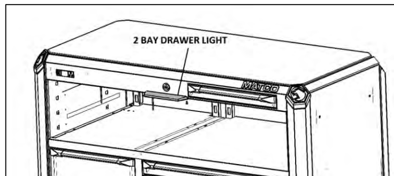
Figure 2- Drawer light is centered in case and installs into preset mounting holes in the case
