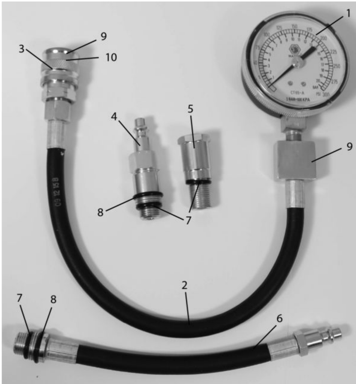
CT66K - COMP.TESTER W/BLOW-MOLD BOX
