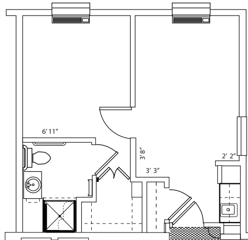
ONE BEDROOM DELUXE 468 SQ FT
