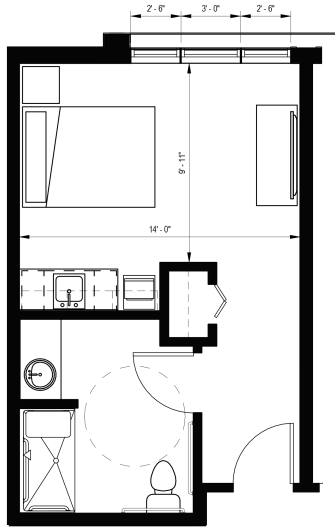
STUDIO 300 SQ FT
