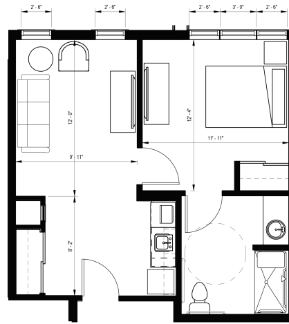
ONE BEDROOM 470 SQ FT
