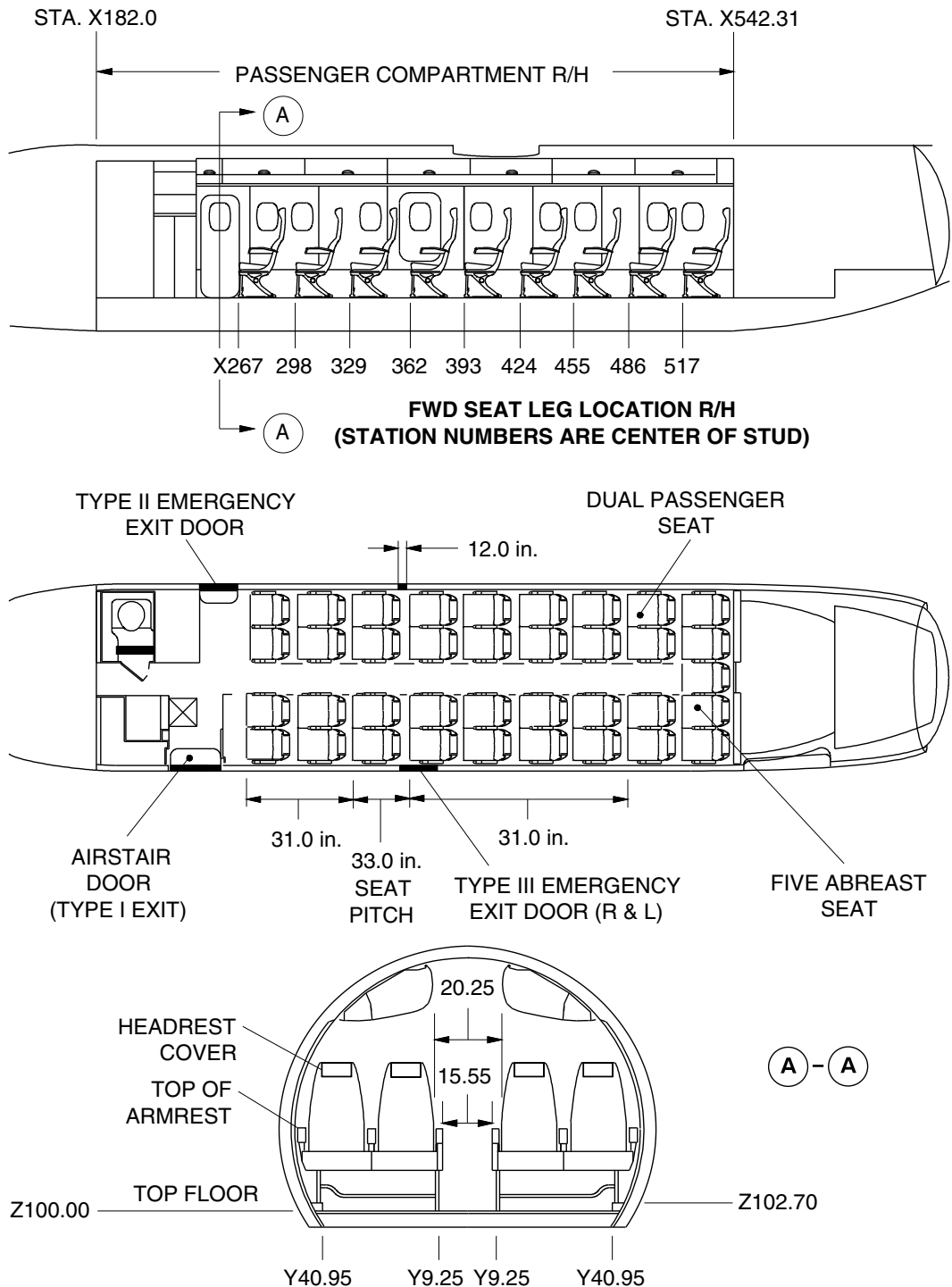
37 Passenger Seats – Description and Operation Figure 1 (Sheet 1 of 2)
