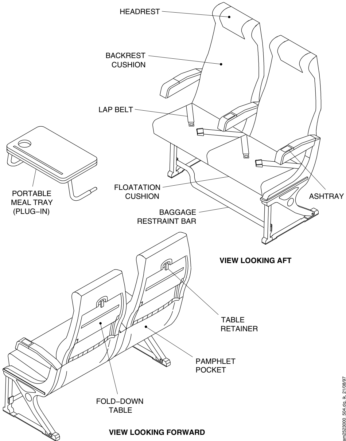
37 Passenger Seats – Description and Operation Figure 1 (Sheet 2 of 2)
