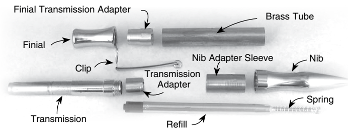
Parts photograph for the Virage ballpoint pen.
