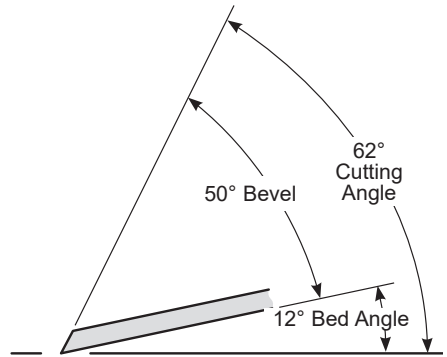
Figure 5: 50° blade geometry.
