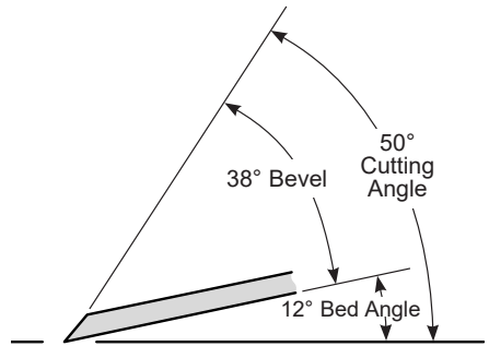
Figure 4: 38° blade geometry.
