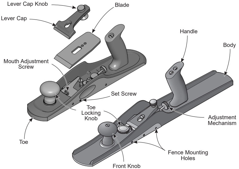
Figure 1: Plane components.
