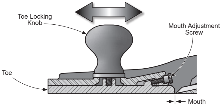
Figure 2: Mouth adjustment.
