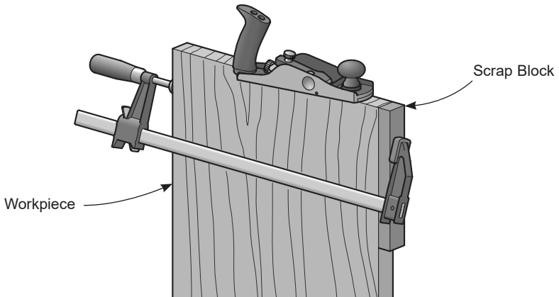
Figure 6: Preventing splitting.
