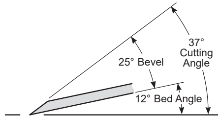
Figure 3: 25° blade geometry.
