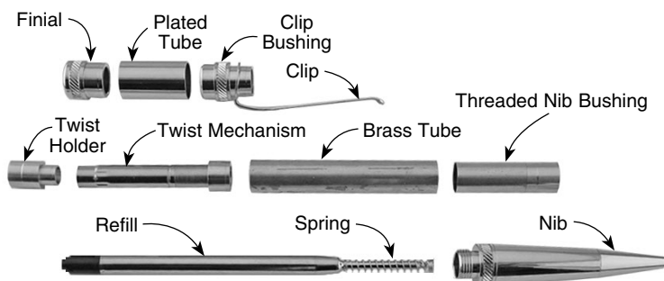
Sierra Diverse ballpoint pen parts.
