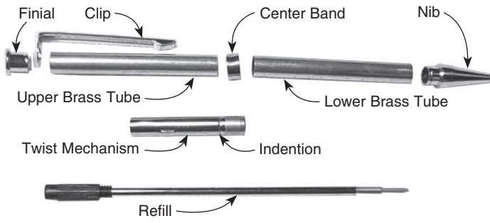
Parts diagram for 7 mm pen.
