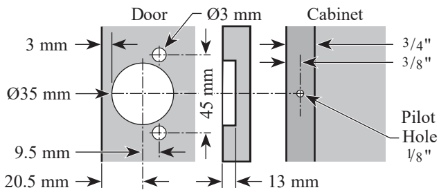
Figure 1: Hole locations.
