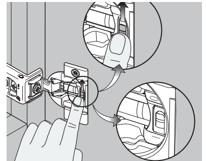
Figure 4: Deactivating the soft-close mechanism.
