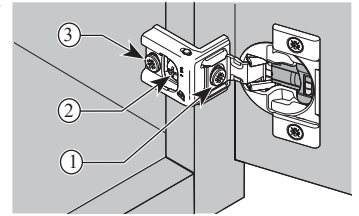
110° Full Overlay Figure 3: Hinge adjustment.
