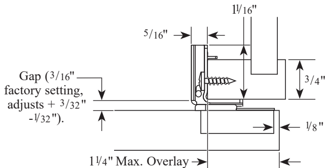
Fig. 2: 110° Compact Clip Full-overlay hinges 1 1/4" (00B1822).
