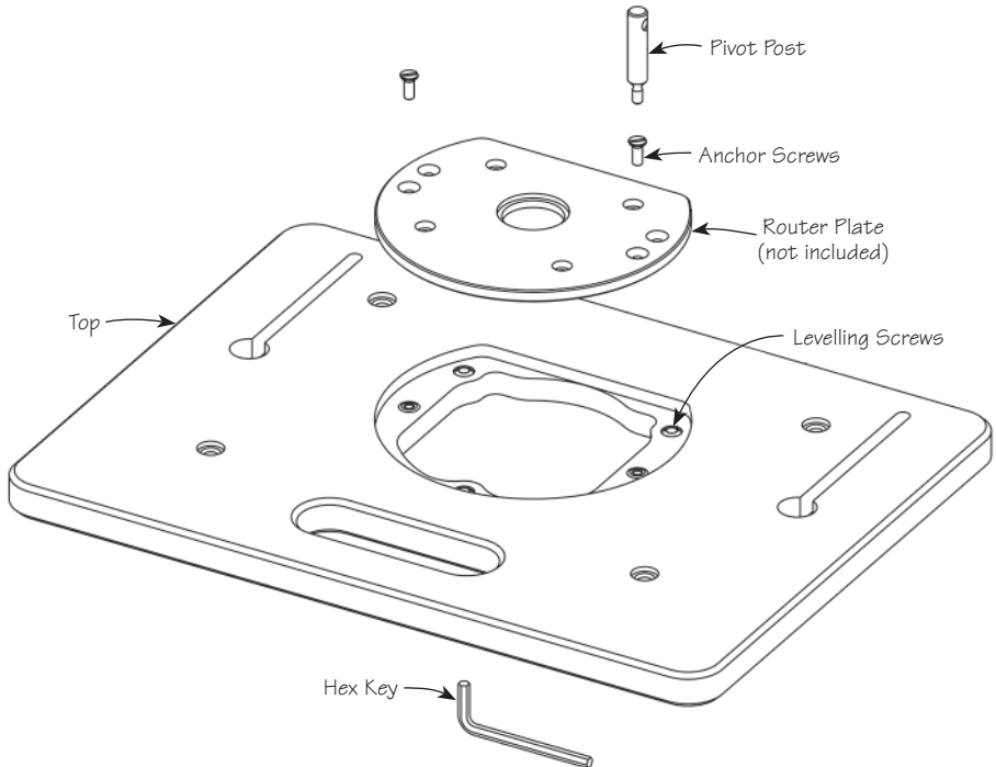
Figure 1: Components of the table top for compact routers.
