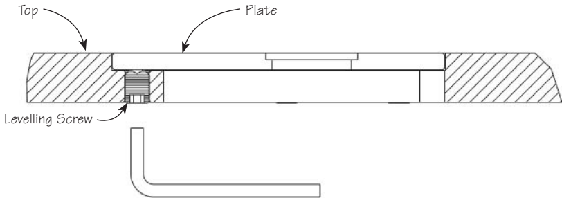
Figure 2: Adjusting the levelling screws.
