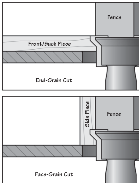
Figure 6: Cut types.
