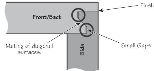
Figure 4: Ideal fit.
