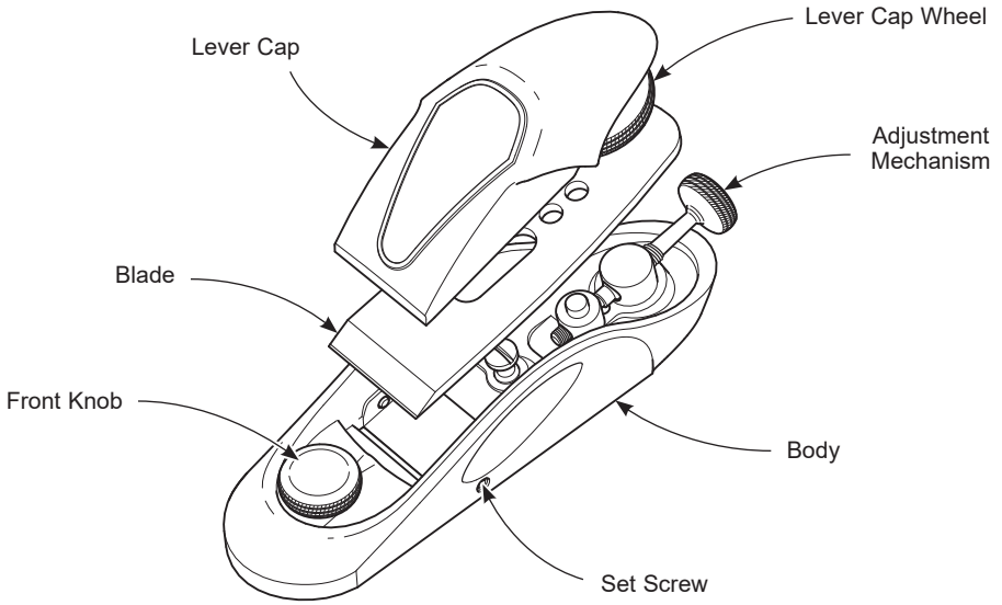
Figure 1: Plane components.
