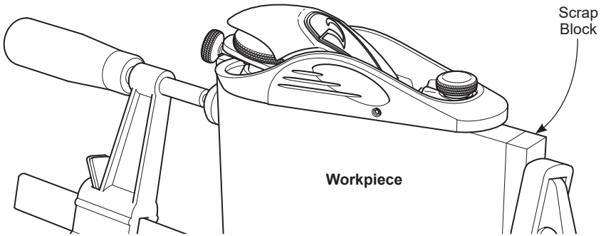
Figure 5: Preventing splitting.
