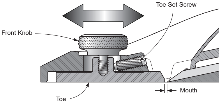
Figure 4: Mouth adjustment.
