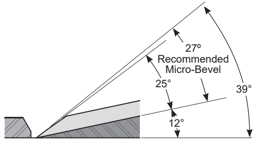
Figure 7: Recommended blade geometry of the low-angle block plane, with a 27° micro-bevel.
