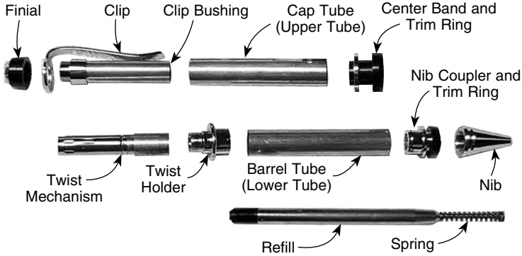
Pen parts.
